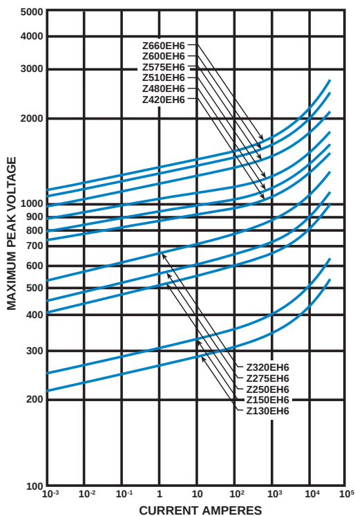
EH Series Voltage VS Current Characteristics
