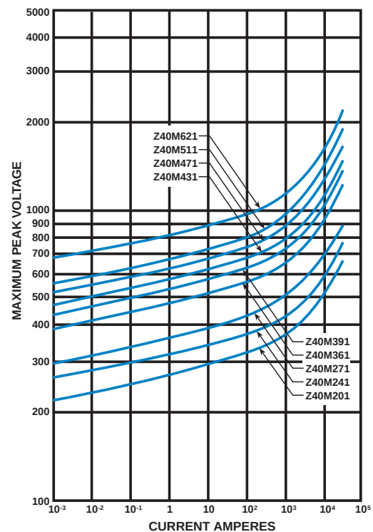
Z40M Series Voltage VS Current Characteristics
