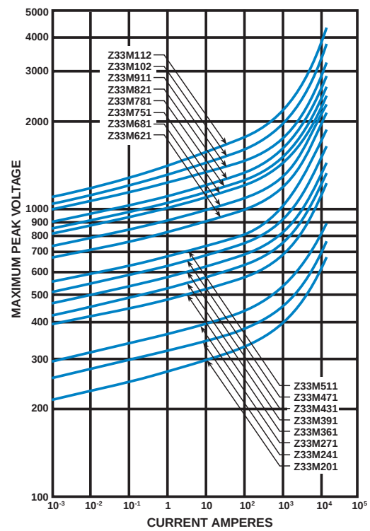
Z33M Series Voltage VS Current Characteristics
