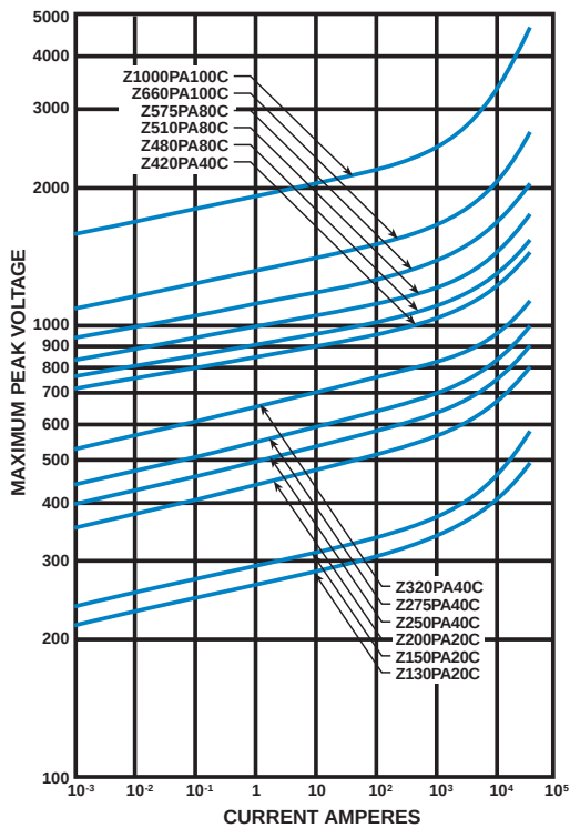
PA Series Voltage VS Current Characteristics
