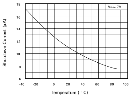
Shutdown Current vs. Temperature
