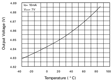
Output Voltage Temperature Coefficient
