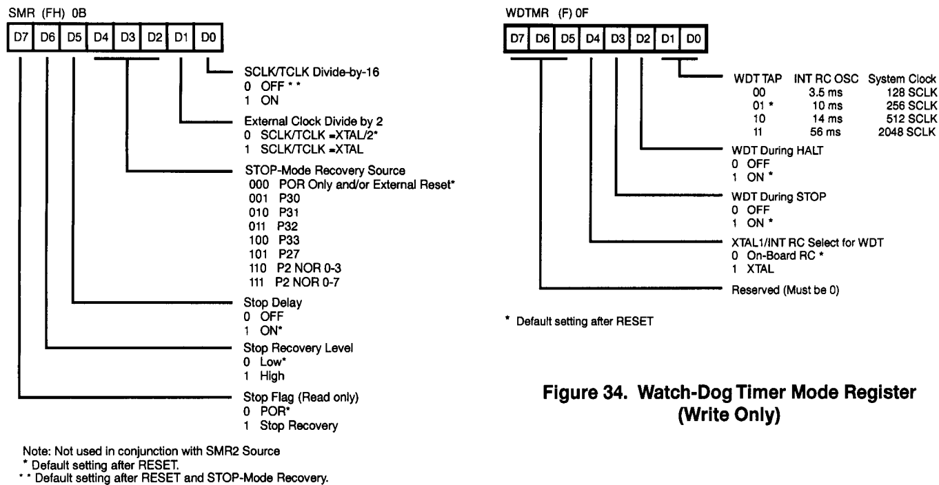
Figure 32. Stop-Mode Recovery Register (Write Only Except Bit D7, Which Is Read Only)
