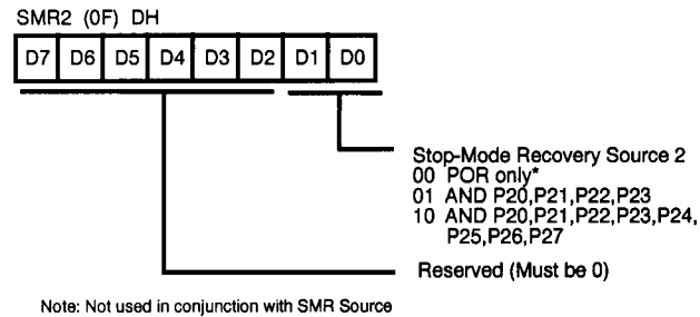
Figure 33. Stop-Mode Recovery Register2
