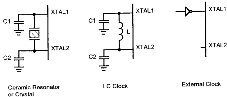
Figure 16. Oscillator Configuration
