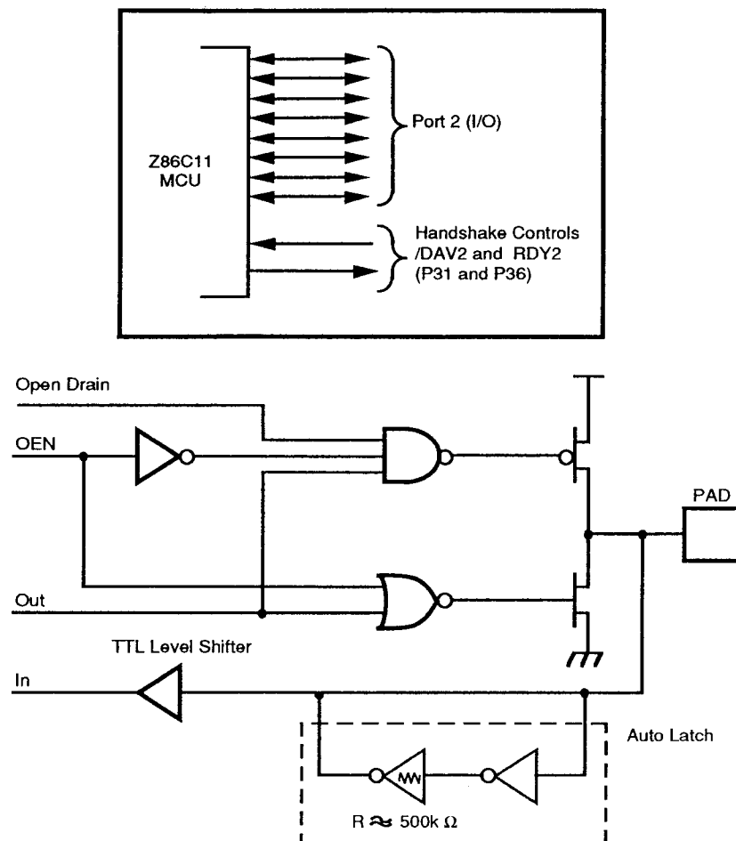
Figure 7. Port 2 Configuration
