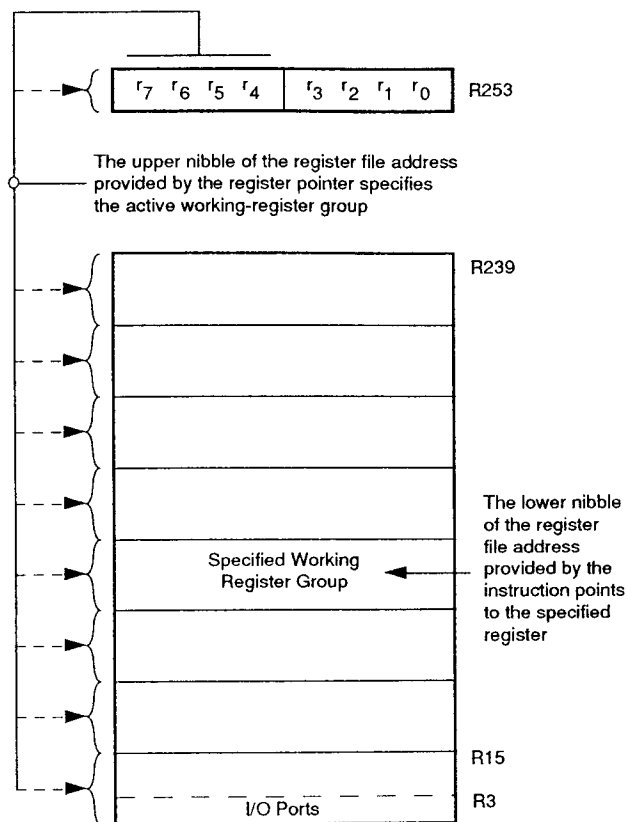
Figure 13. Register Pointer
