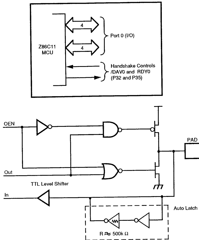
Figure 5. Port 0 Configuration
