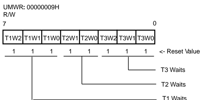
Figure 41. Upper Memory Waits Register
