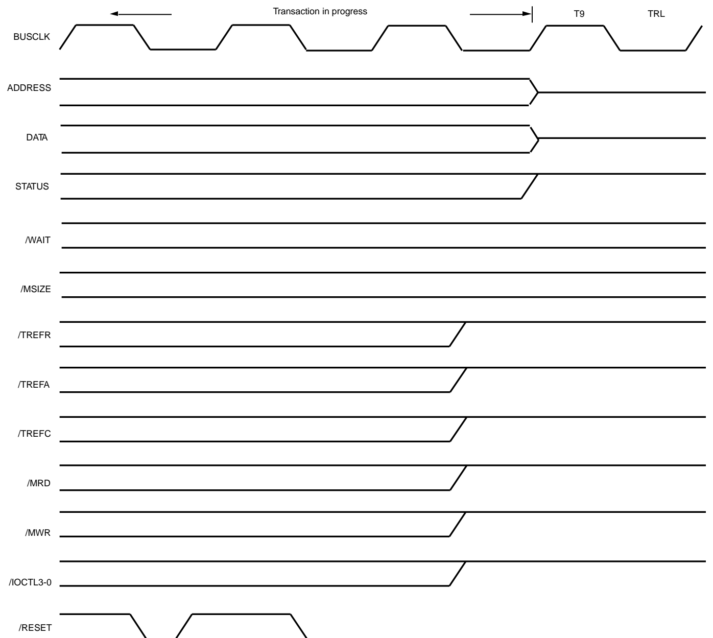
Figure 18. Reset Entry
