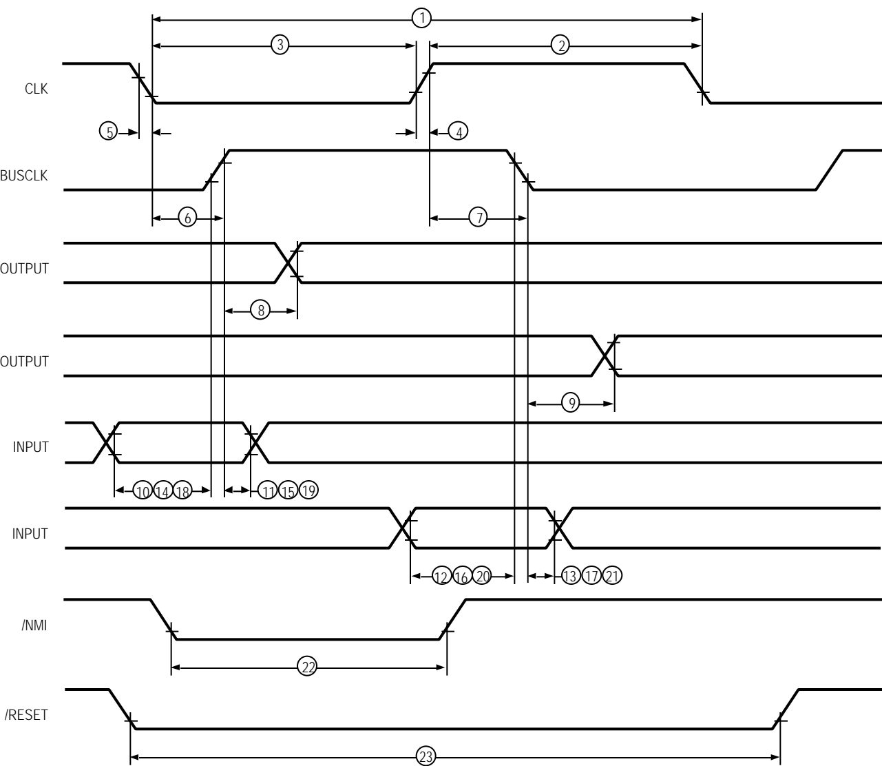
Figure 56. Z380™ CPU Timing
