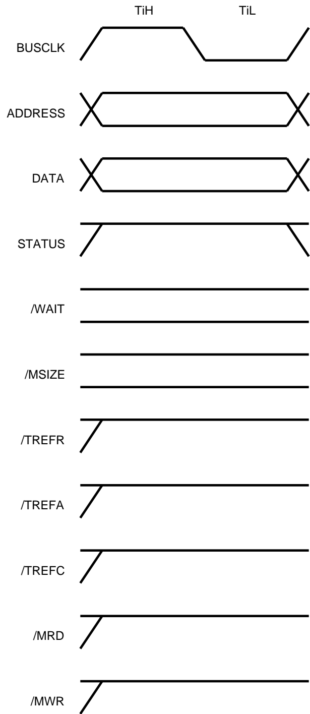
Figure 16. Idle Cycle
