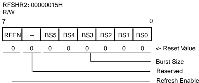
Figure 49. Refresh Register 2
