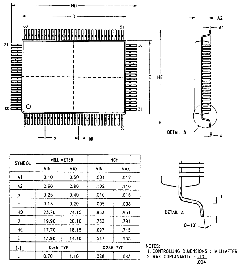
100-Lead QFP Package Diagram
