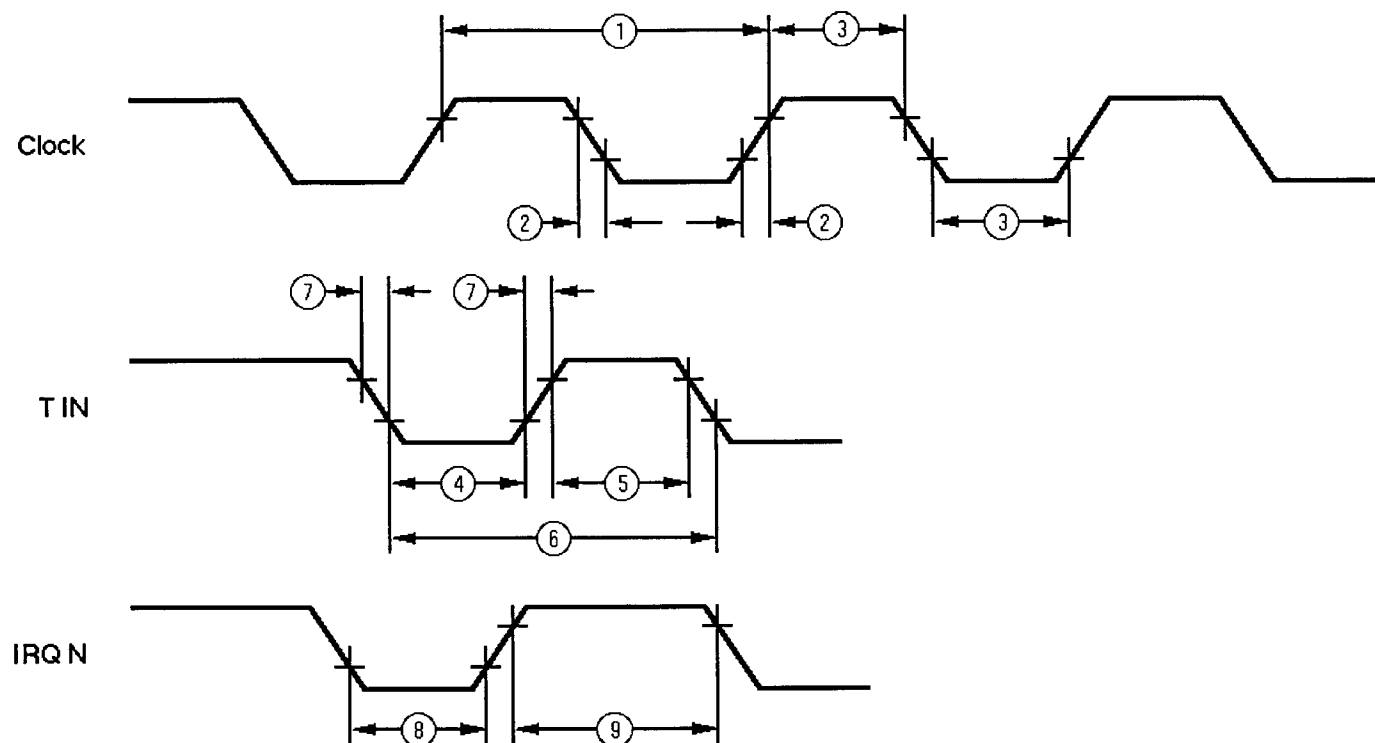
Figure 9. Additional Timing
