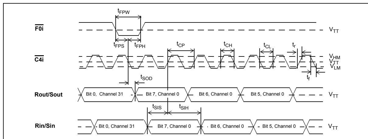
Figure 12 - ST-BUS Timing at 2.048 Mbps
