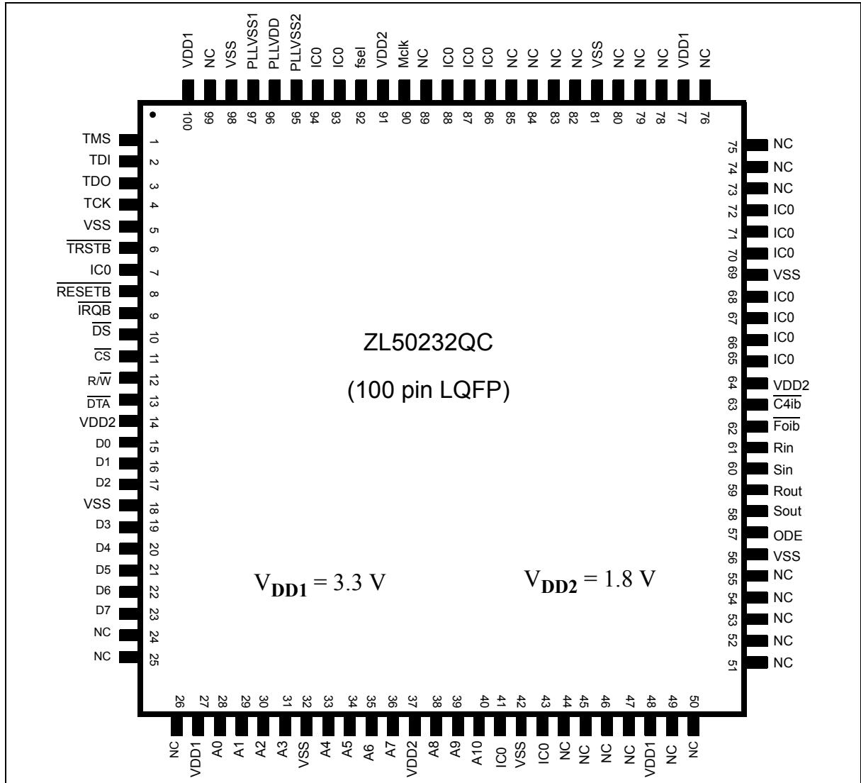
Figure 2 - 100 Pin LQFP
