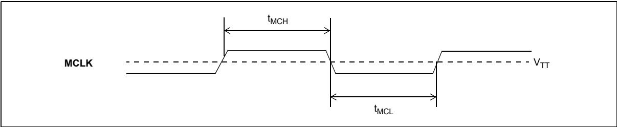
Figure 14 - Master Clock
