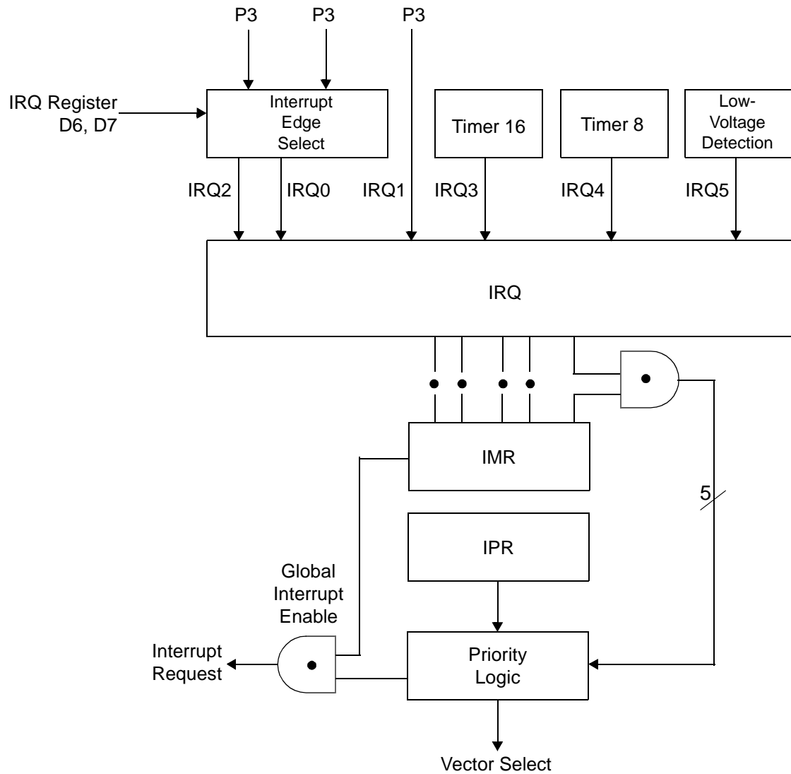
Figure 30. Interrupt Block Diagram
