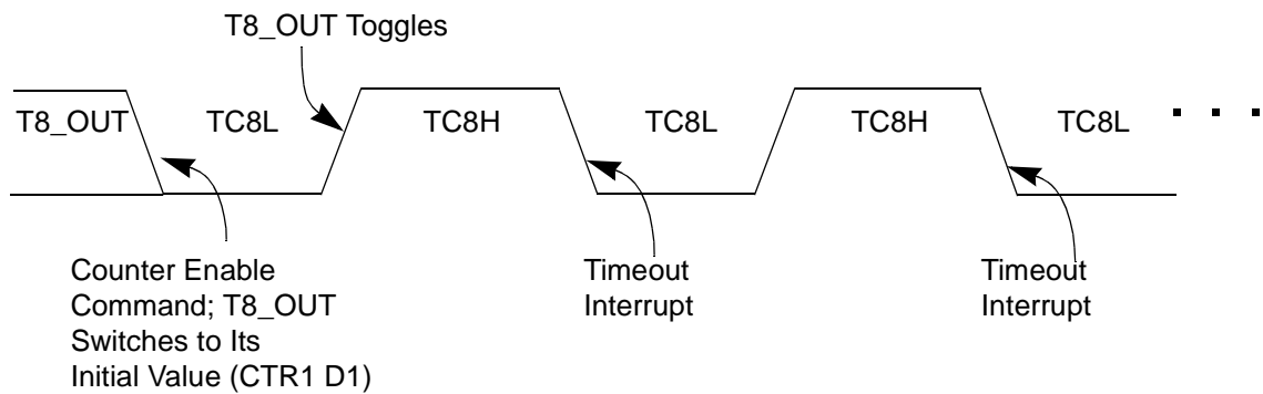
Figure 22. T8_OUT in Modulo-N Mode
