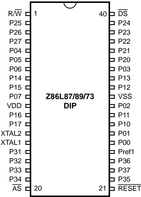
Figure 3. 40-Pin DIP Pin Assignment
