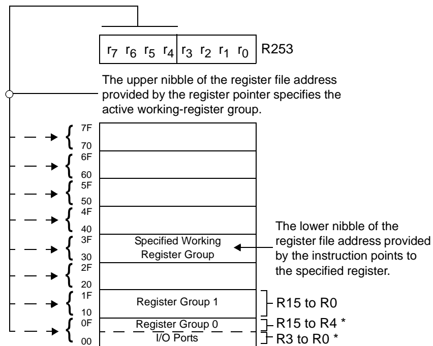
Figure 17. Register Pointer—Detail
