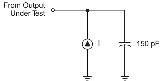
Figure 6. Test Load Diagram
