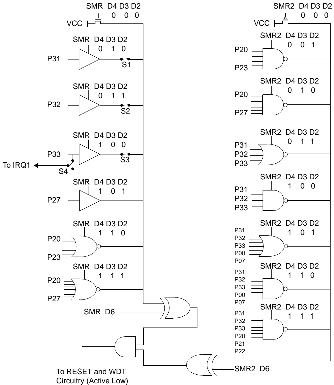
Figure 35. Stop-Mode Recovery Source
