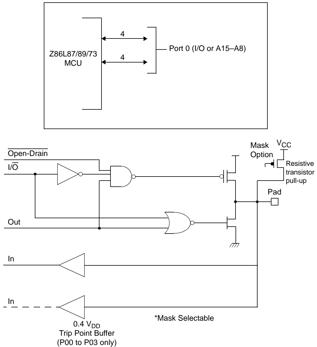
Figure 9. Port 0 Configuration
