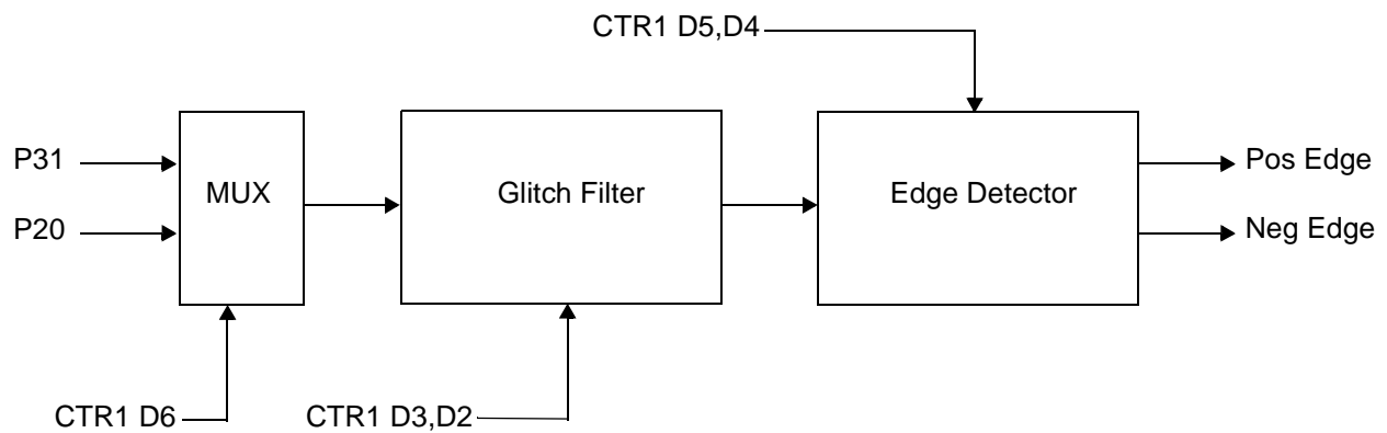
Figure 18. Glitch Filter Circuitry
