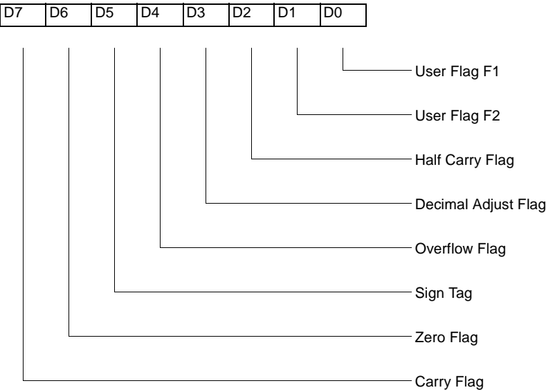
Figure 53. Flag Register (FCh: Read/Write)
