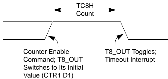
Figure 21. T8_OUT in Single-Pass Mode
