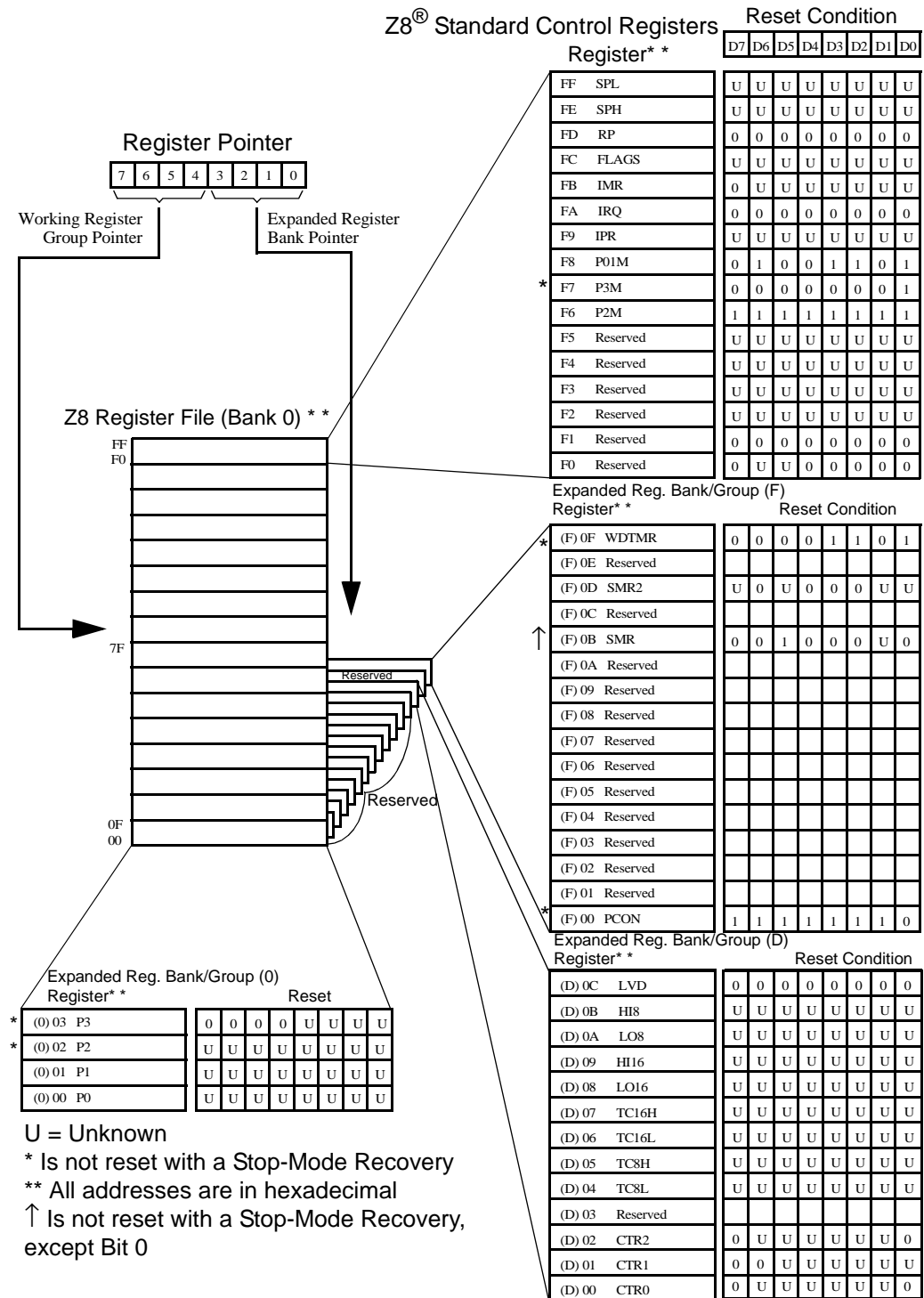
Figure 15. Expanded Register File Architecture
