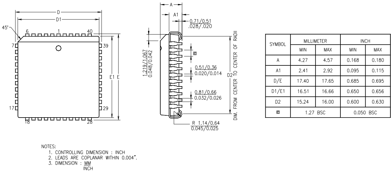
Figure 58. 44-Pin PLCC Package Diagram
