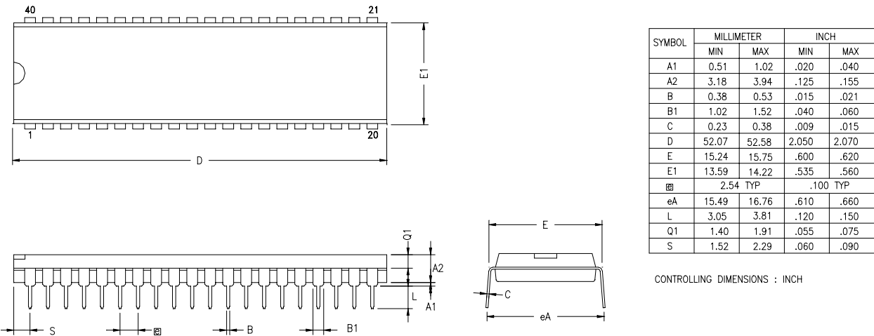
Figure 57. 40-Pin DIP Package Diagram
