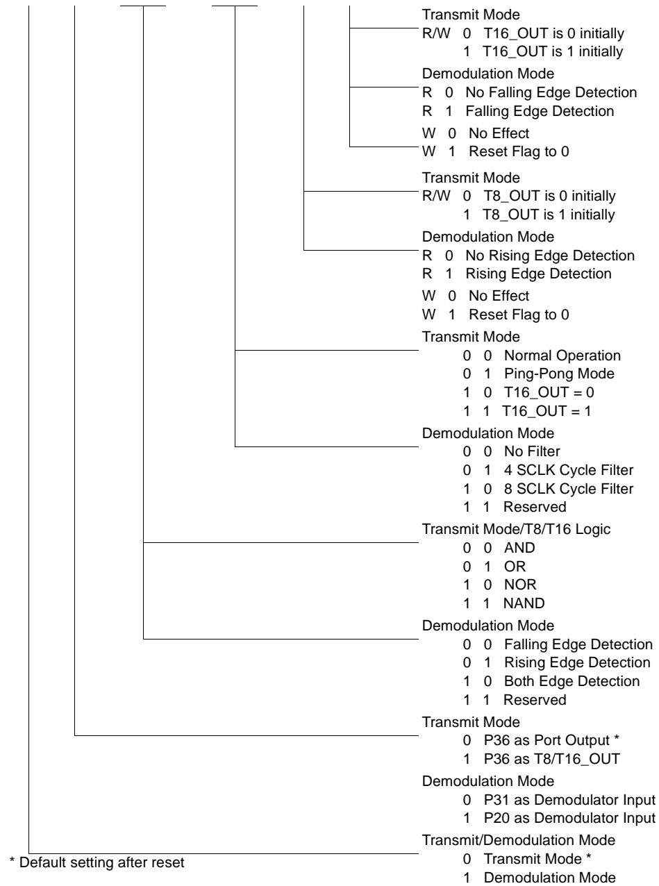
Figure 40. T8 and T16 Common Control Functions ((0D) 1h: Read/Write)
