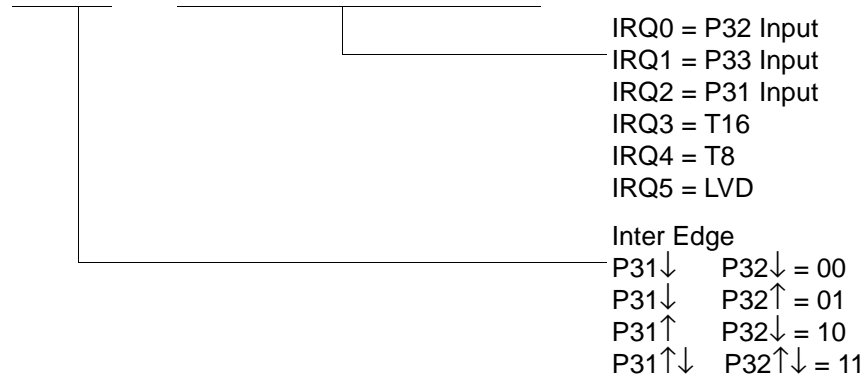
Figure 51. Interrupt Request Register (FAh: Read/Write)
