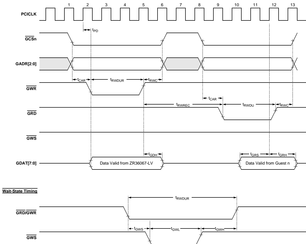
Figure 13. GuestBus Timing
