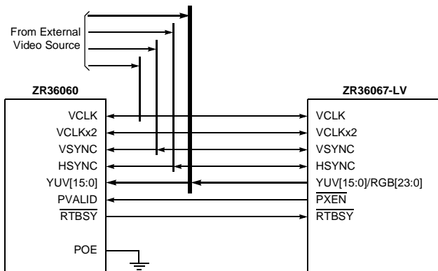
Figure 3. Recommended Connection of ZR36067-LV to ZR36060 Video Interface
