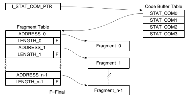
Figure 9. JPEG Code Data Structure In System Memory
