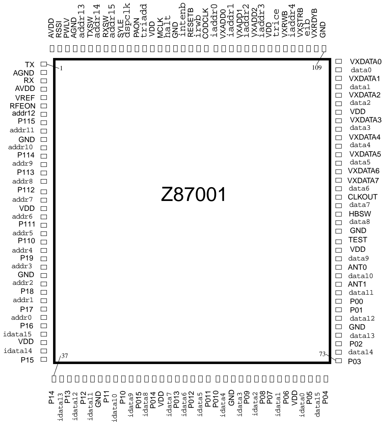
Figure 3. 144 Pin VQFP Pin Configuration
