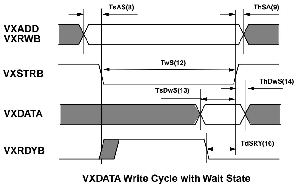
Figure 8. Read/Write Cycle Timing with Wait State
