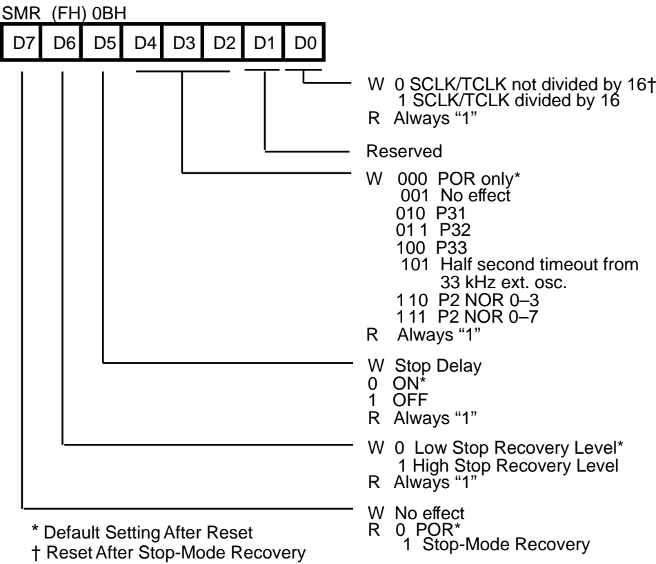
Figure 59. Stop-Mode Recovery Register (SMR) (F) 0BH [Read/Write]
