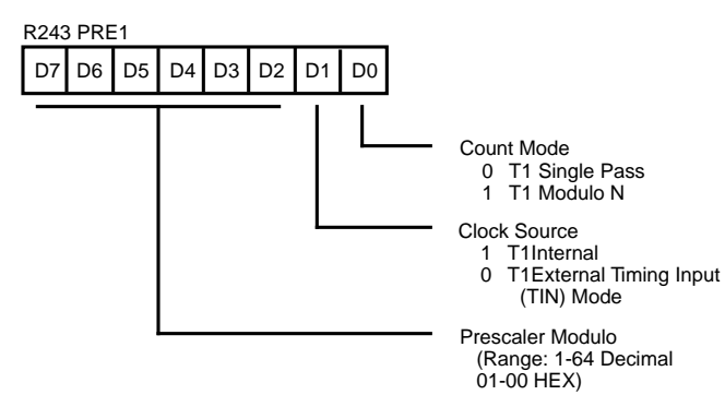
Figure 66. Prescaler 0 Register (F5H: Write-Only)
