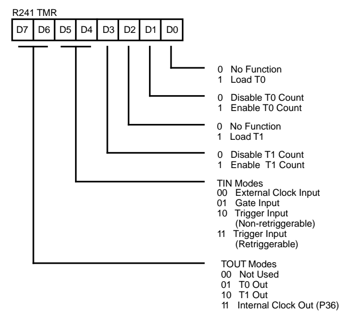
Figure 62. Timer Mode Register (F1H: Read/Write)
