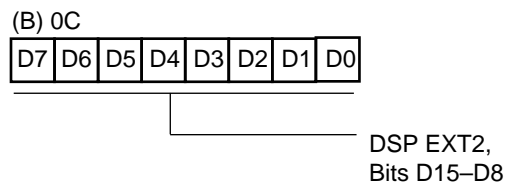
Figure 49. Incoming Register from DSP EXT2 (High Byte) (B) 0CH [Read-Only]
