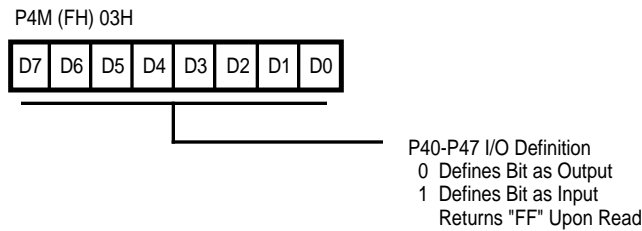
Figure 55. Port 4 Mode Register (F) 03H [Write-Only]
