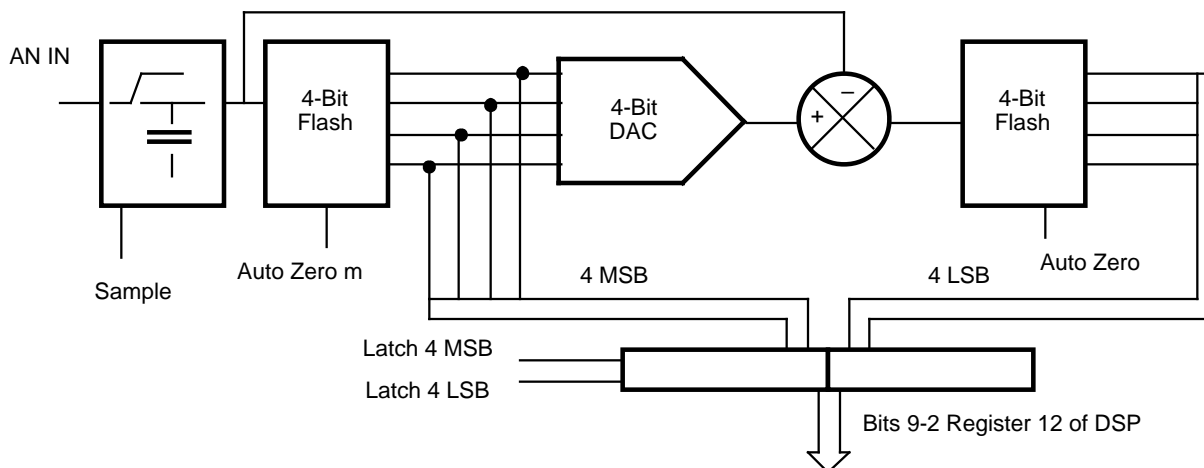
Figure 34. A/D Converter
