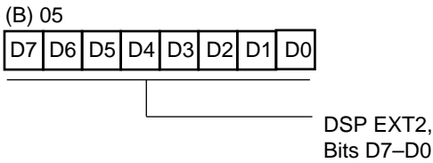
Figure 42. Outgoing Register to DSP EXT2 (Low Byte) (B) 05H [Read/Write]
