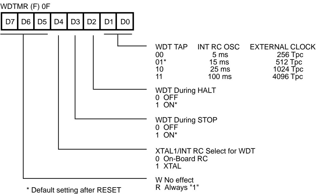
Figure 22. Watch-Dog Timer Mode Register
