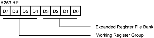
Figure 74. Register Pointer (FDH: Read/Write)
