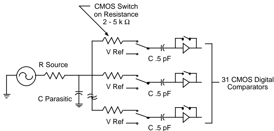
Figure 36. Input Impedance of ADC
