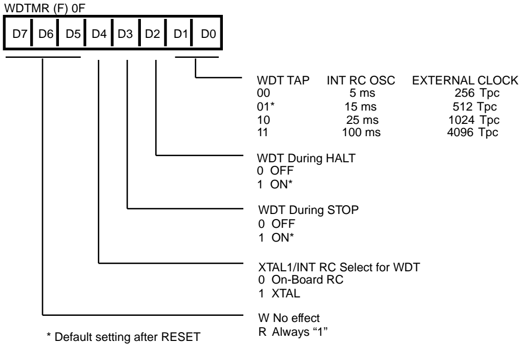
Figure 60. Watch-Dog Timer Mode Register (F) 0FH [Read/Write]
