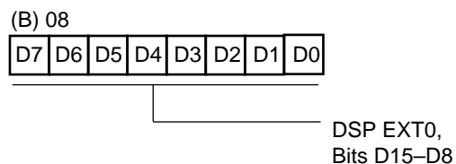
Figure 45. Incoming Register from DSP EXT0 (High Byte) (B) 08H [Read-Only]
