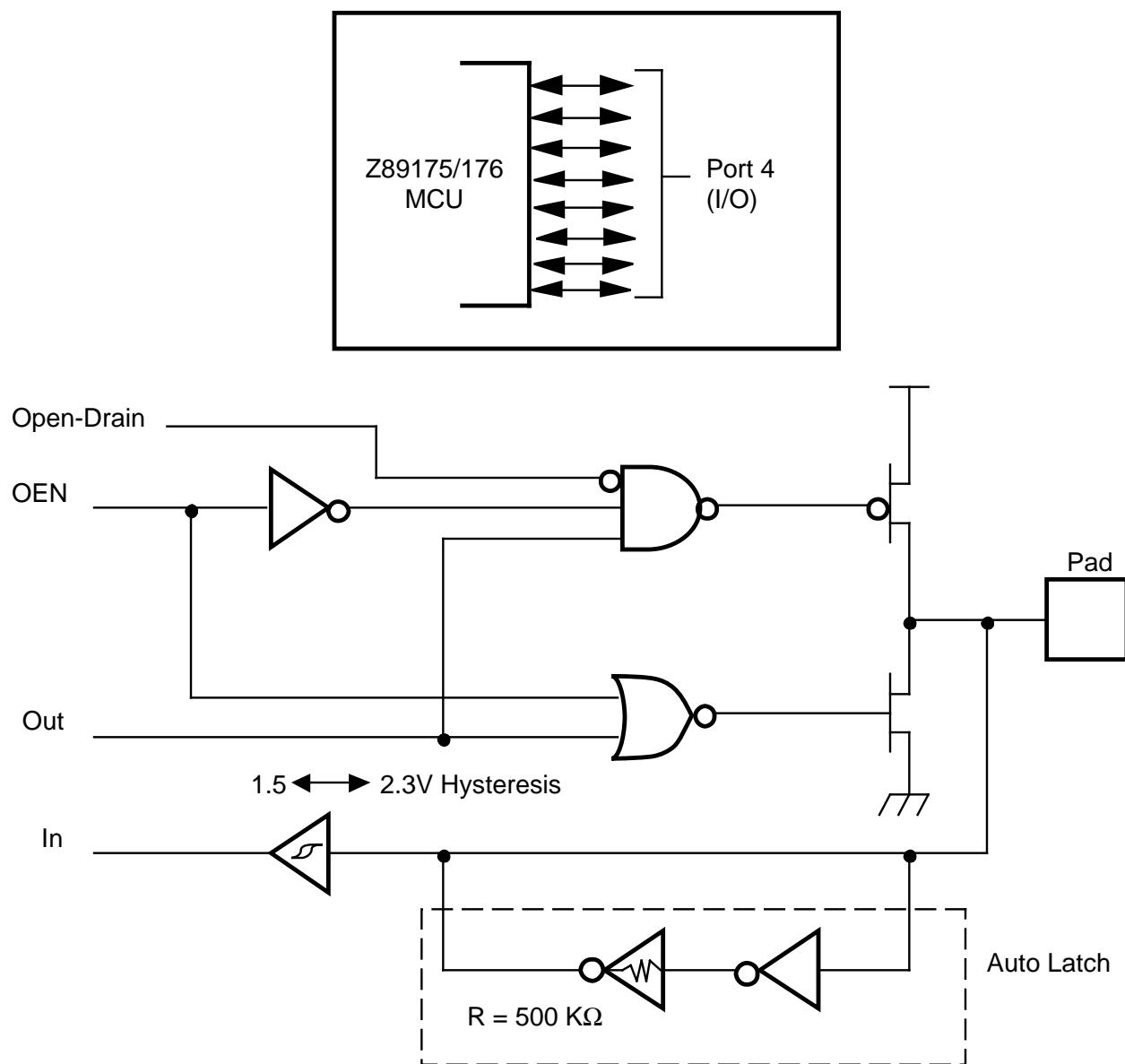
Figure 10. Port 4 Configuration
