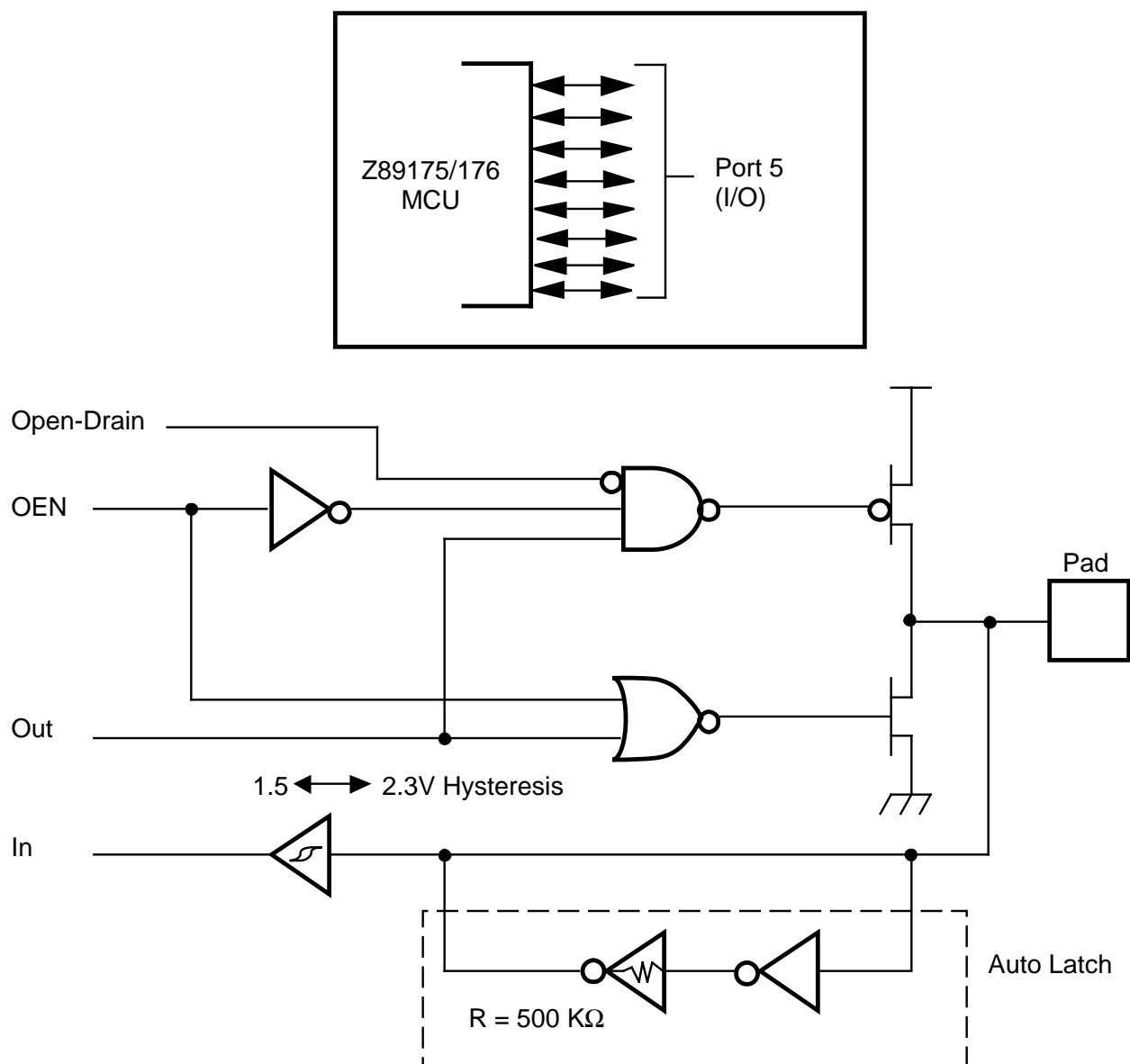
Figure 11. Port 5 Configuration
