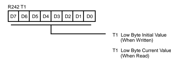
Figure 63. Counter/Timer 1 Register (F2H: Read/Write)
