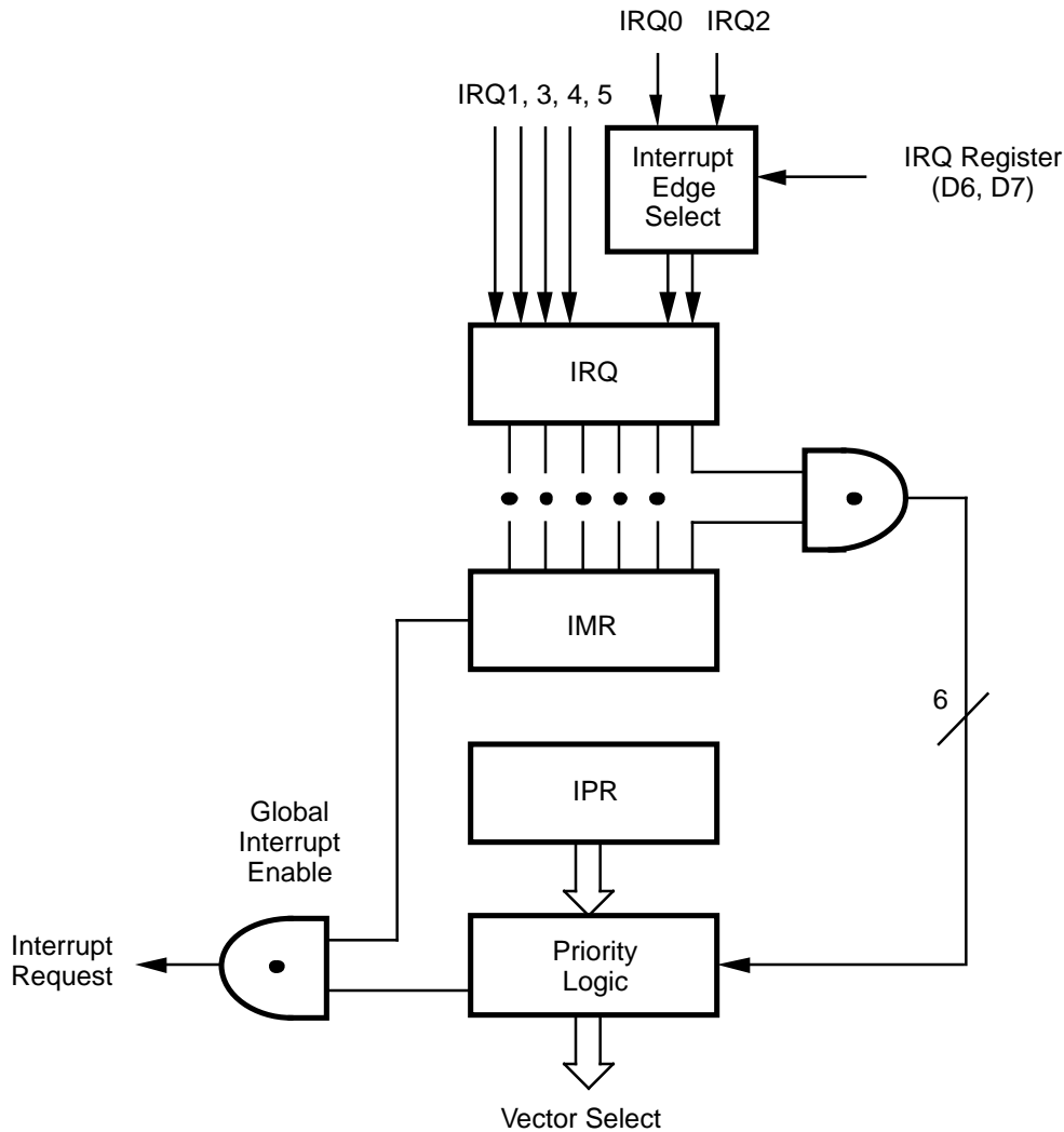
Figure 16. Interrupt Block Diagram
