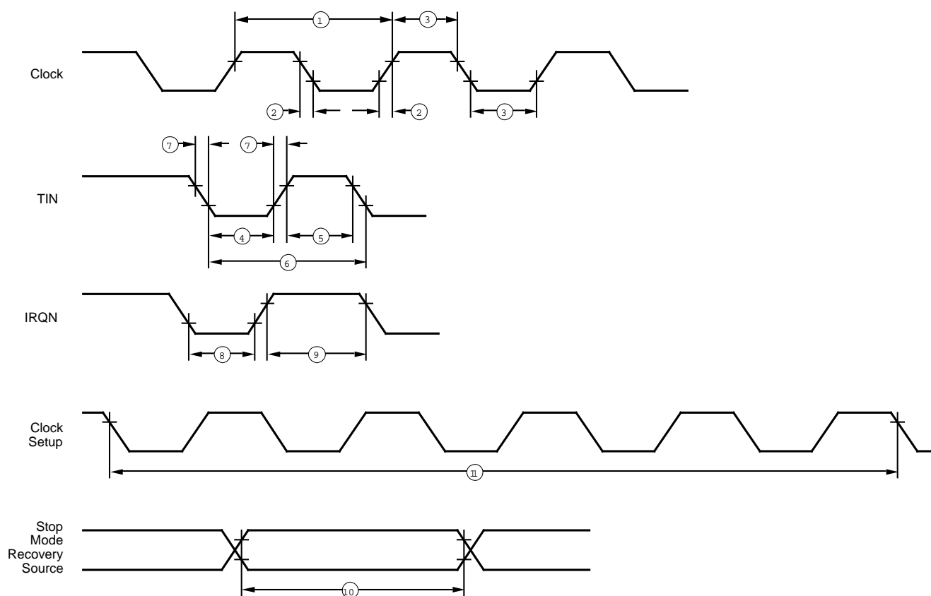
Figure 5. Additional Timing
