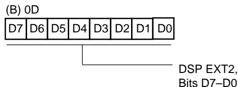
Figure 50. Incoming Register from DSP EXT2 (Low Byte) (B) 0DH [Read-Only]
