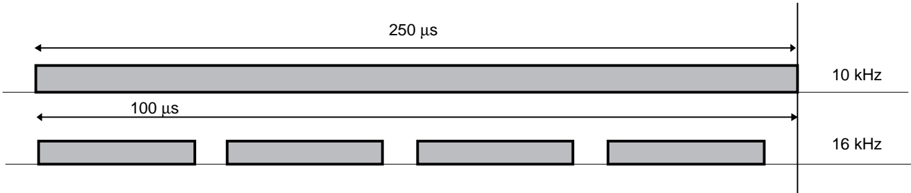
Figure 32. PWM Waveform (shaded area indicates the active region)
