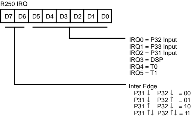
Figure 71. Interrupt Request Register (FAH: Read/Write)
