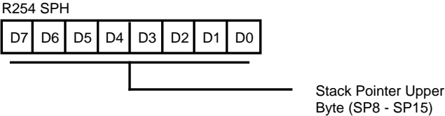
Figure 75. Stack Pointer High (FEH: Read/Write)
