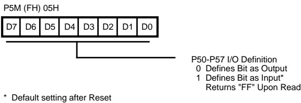
Figure 57. Port 5 Mode Register (F) 05H [Write-Only]
