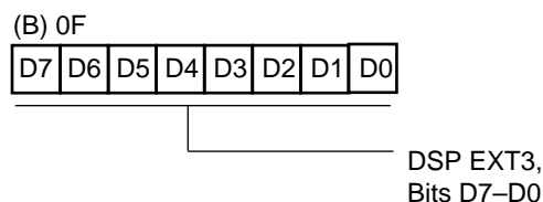
Figure 52. Incoming Register from DSP EXT3 (Low Byte) (B) 0FH [Read-Only]
