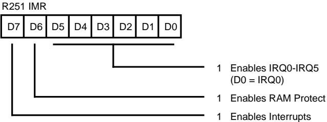
Figure 72. Interrupt Mask Register (FBH: Read/Write)
