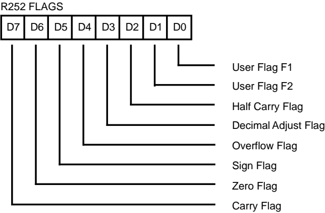
Figure 73. Flag Register (FCH: Read/Write)
