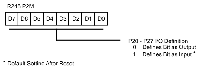
Figure 67. Port 2 Mode Register (F6H: Write-Only)
