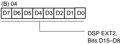
Figure 41. Outgoing Register to DSP EXT2 (High Byte) (B) 04H [Read/Write]
