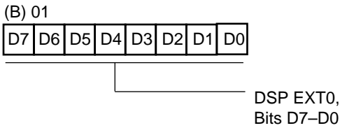
Figure 38. Outgoing Register to DSP EXT0 (Low Byte) (B) 01H [Read/Write]
