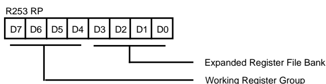
Figure 13. Register Pointer Register
