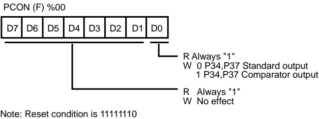
Figure 19. Port Configuration Register (PCON)
