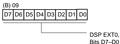
Figure 46. Incoming Register from DSP EXT0 (Low Byte) (B) 09H [Read-Only]
