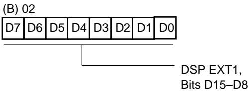
Figure 39. Outgoing Register to DSP EXT1 (High Byte) (B) 02H [Read/Write]
