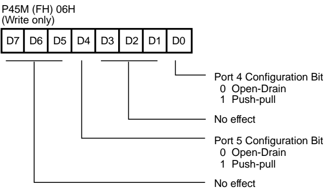
Figure 58. Port 4 and 5 Configuration Register (F) 06H [Write-Only]
