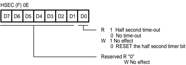
Figure 23. Half-Second Timer Status Register
