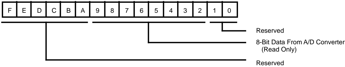
Figure 30. EXT5 Register A/D Mode Definition
