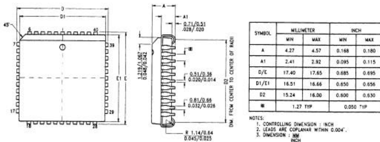
Figure 77. 44-Pin PLCC Package Diagram
