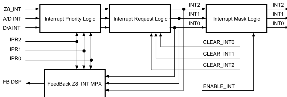
Figure 26. DSP Interrupts
