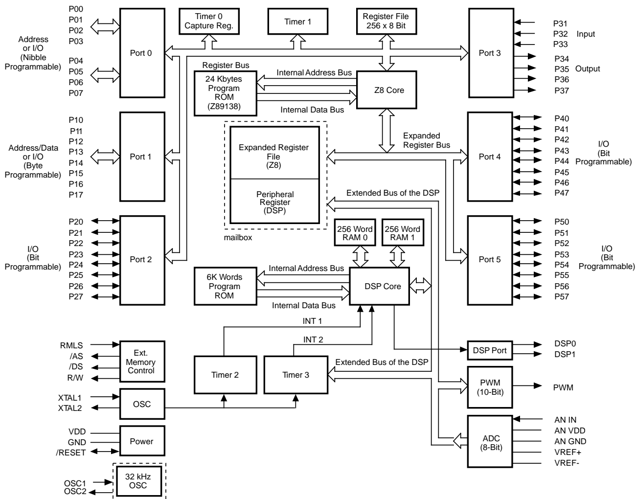
Figure 1. Z89140 Functional Block Diagram
