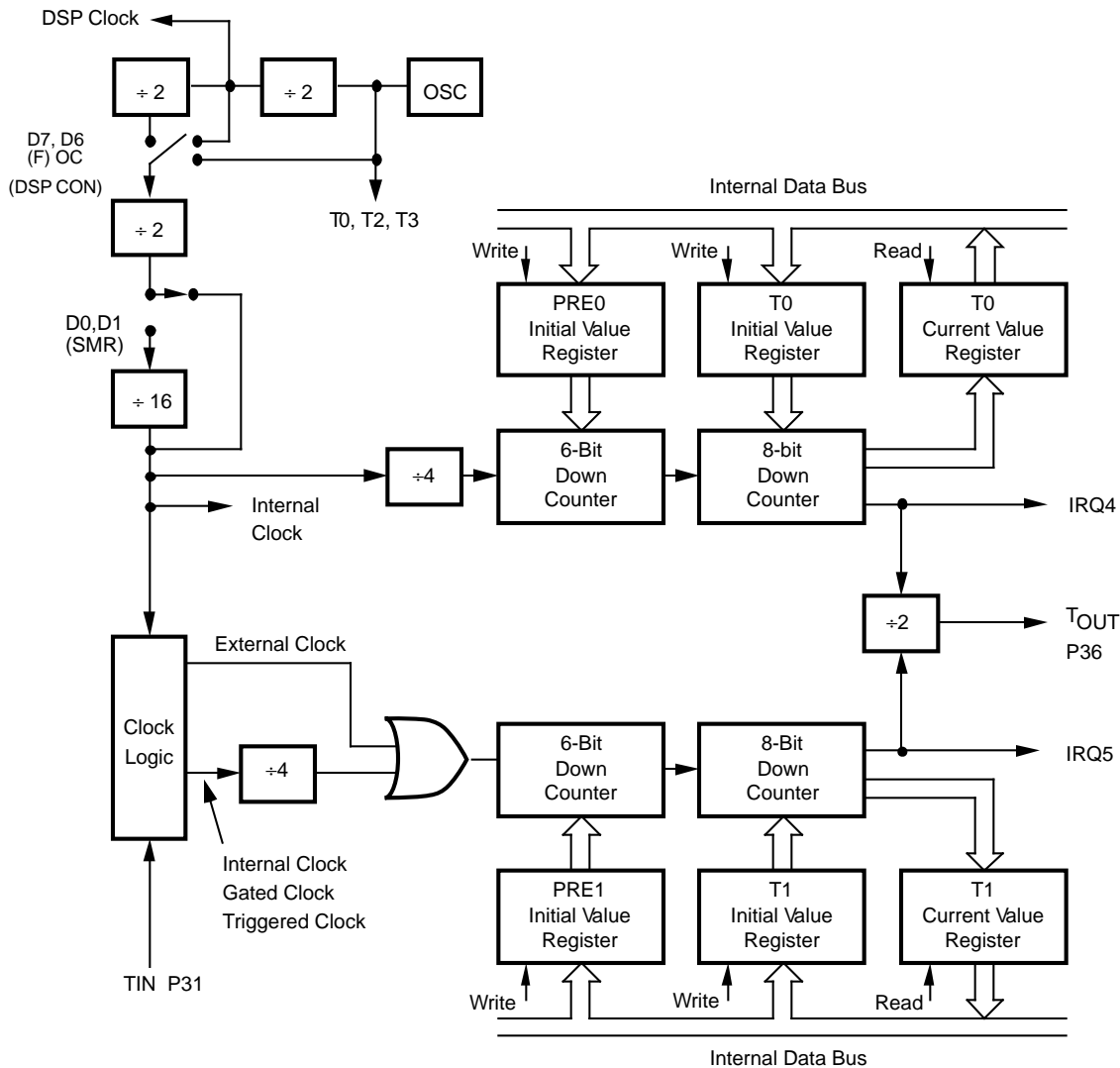
Figure 18. Counter/Timer Block Diagram
