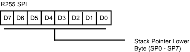
Figure 76. Stack Pointer Low (FFH: Read/Write)
