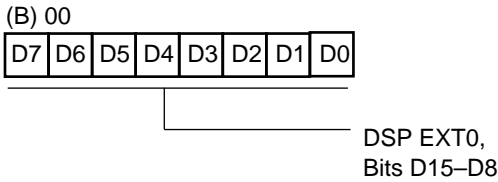
Figure 37. Outgoing Register to DSP EXT0 (High Byte) (B) 00H [Read/Write]
