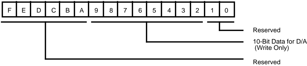
Figure 29. EXT5 Register D/A Mode Definition
