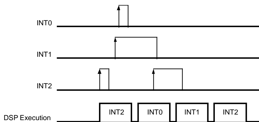
Figure 27. DSP Interrupt Priority Structure
