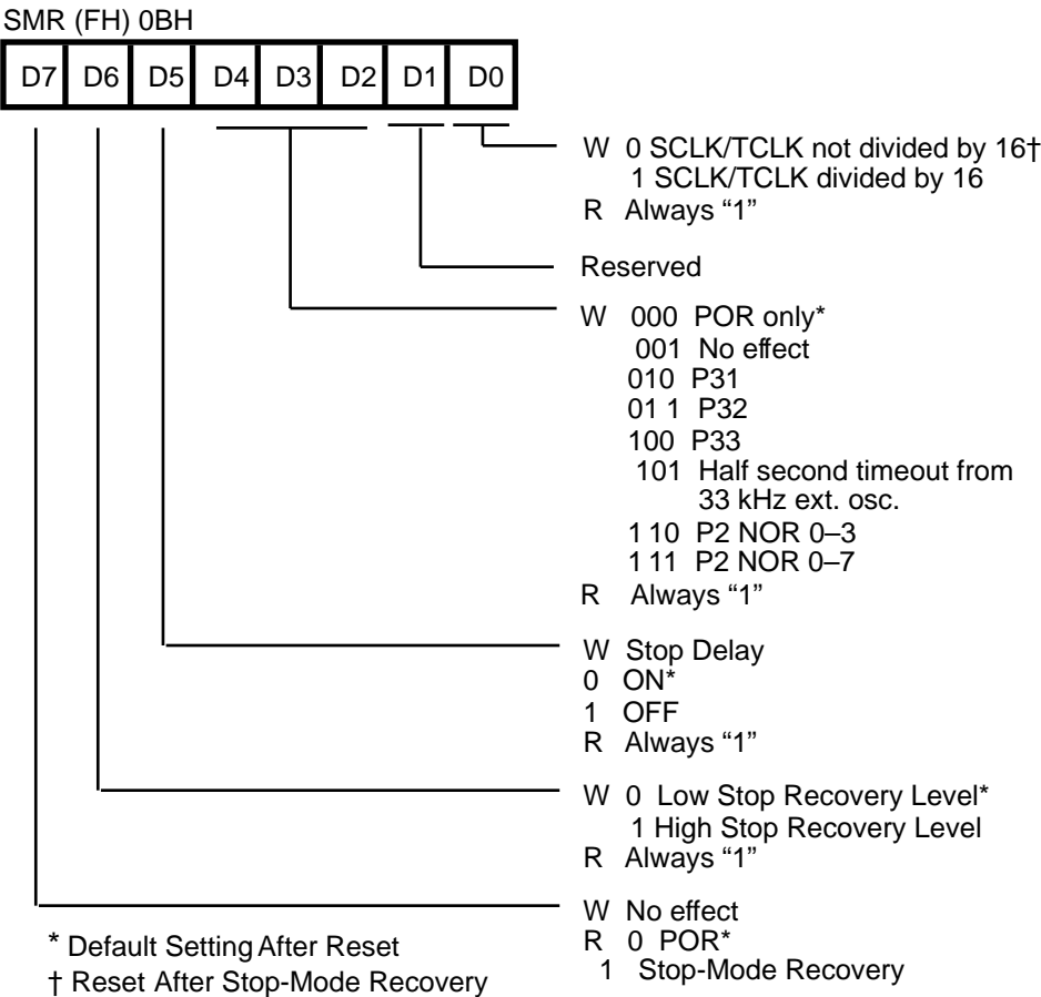
Figure 20. Stop-Mode Recovery Register (SMR)
