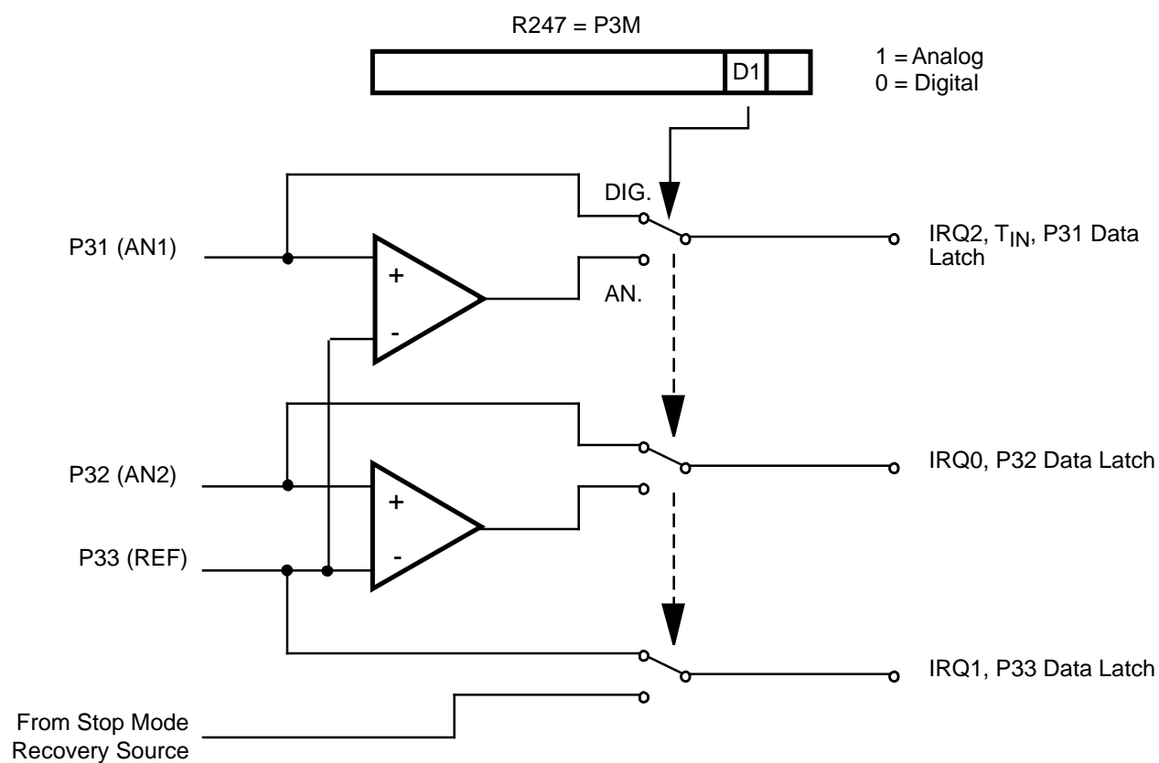
Figure 9. Port 3 Configuration
