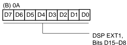
Figure 47. Incoming Register from DSP EXT1 (High Byte) (B) 0AH [Read-Only]
