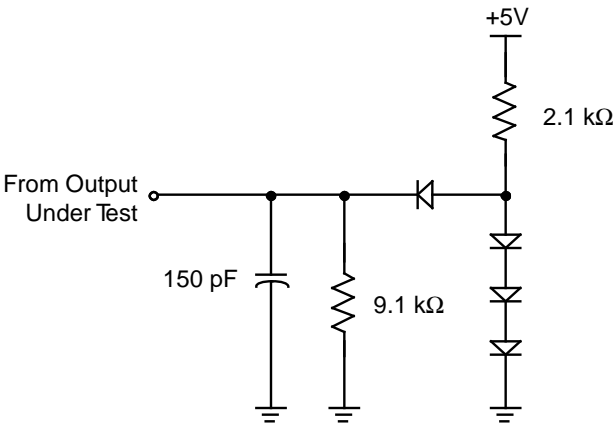
Figure 4. Test Load Diagram
