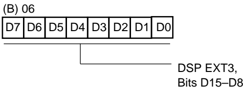
Figure 43. Outgoing Register to DSP EXT3 (High Byte) (B) 06H [Read/Write]
