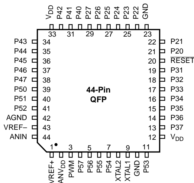
Figure 3. Z89140 44-Pin QFP Pin Configuration
