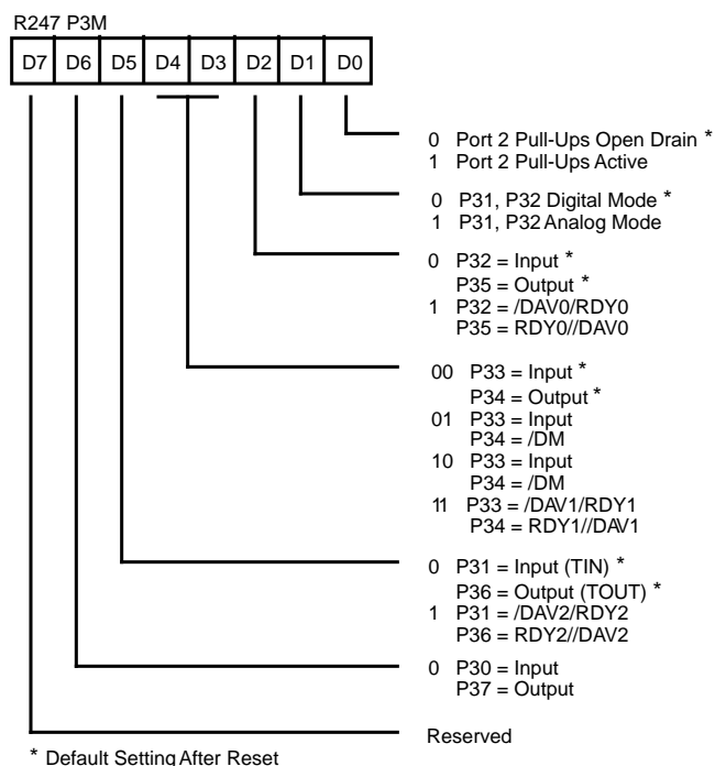
Figure 68. Port 3 Mode Register (F7H: Write-Only)
