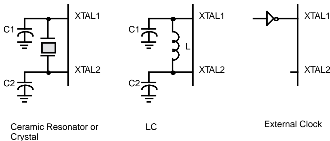
Figure 17. Oscillator Configuration
