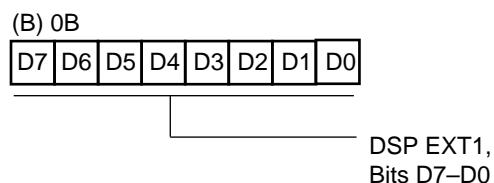
Figure 48. Incoming Register from DSP EXT1 (Low Byte) (B) 0BH [Read-Only]
