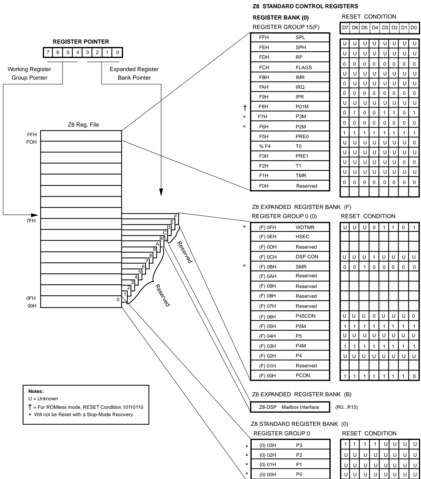
Figure 15. Expanded Register File Architecture
