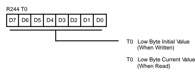
Figure 65. Counter/Timer 0 Register (F4H: Read/Write)
