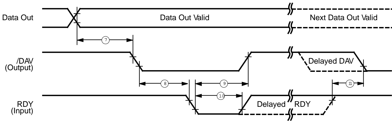
Figure 7. Output Handshake Timing
