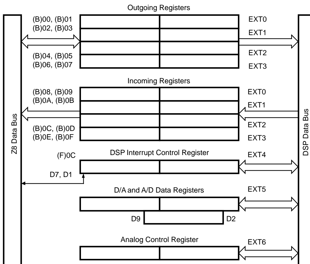
Figure 25. Z8-DSP Interface
