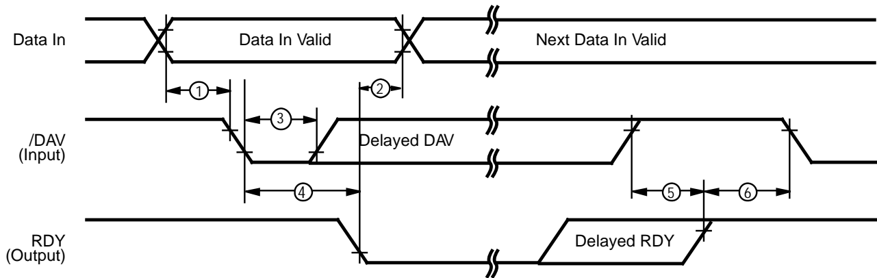
Figure 6. Input Handshake Timing
