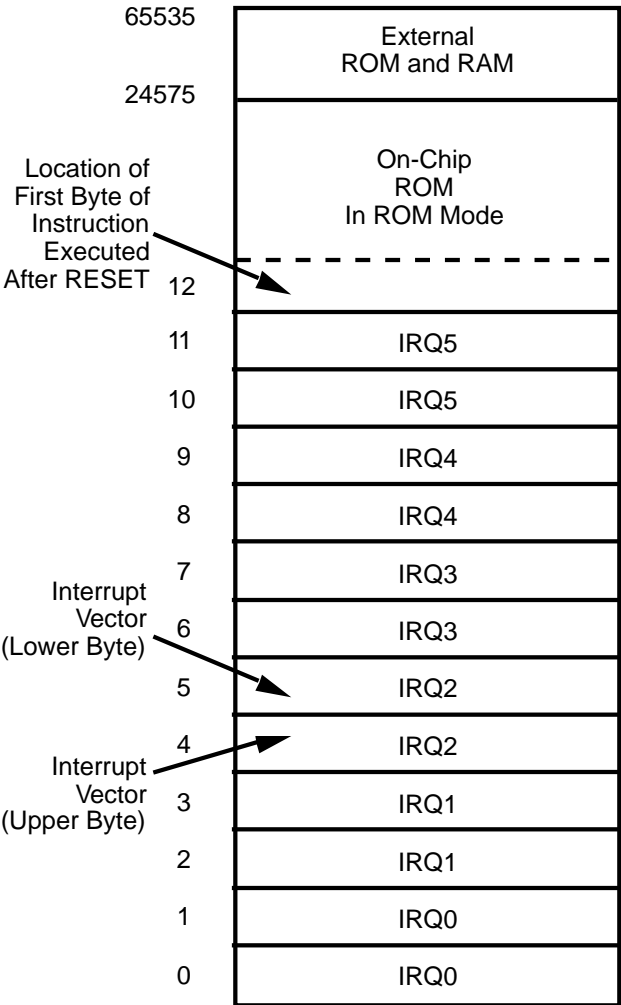
Figure 12. Program Memory
