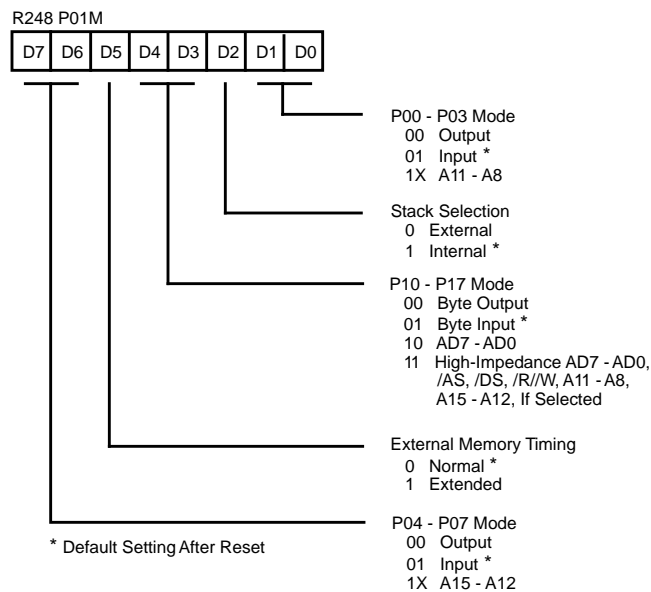
Figure 69. Port 0 Mode Register (F8H: Write-Only)
