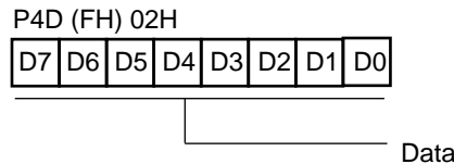
Figure 53. Port Configuration Register (PCON) (F) 00H [Write-Only]
