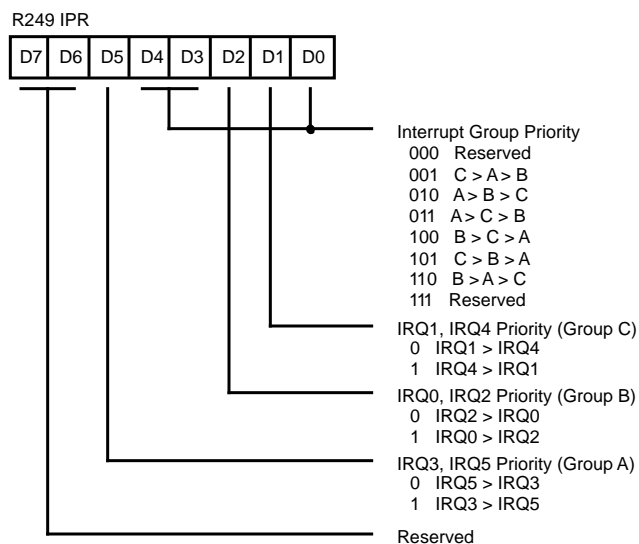
Figure 70. Interrupt Priority Register (F9H: Write-Only)
