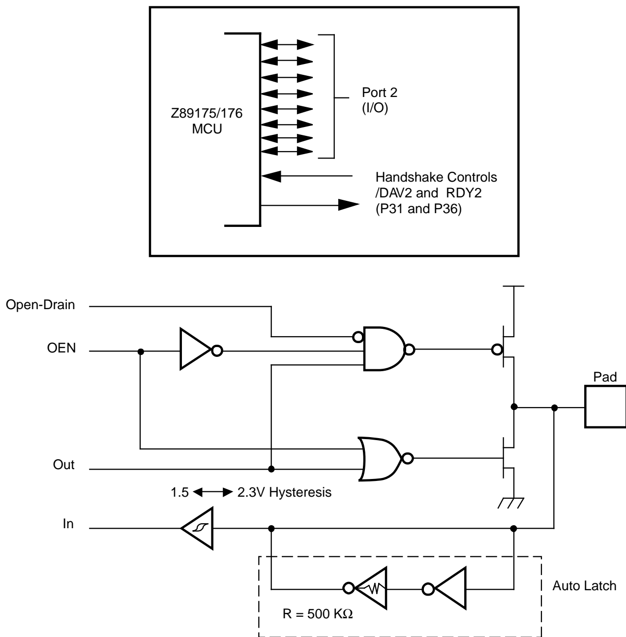
Figure 8. Port 2 Configuration
