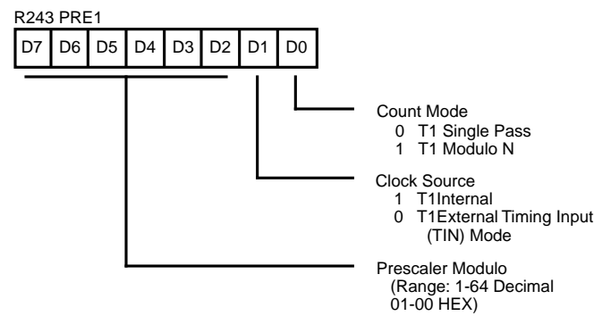
Figure 64. Prescaler 1 Register (F3H: Write-Only)
