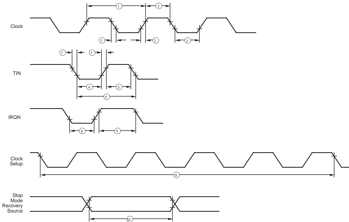
Figure 8. Additional Timing
