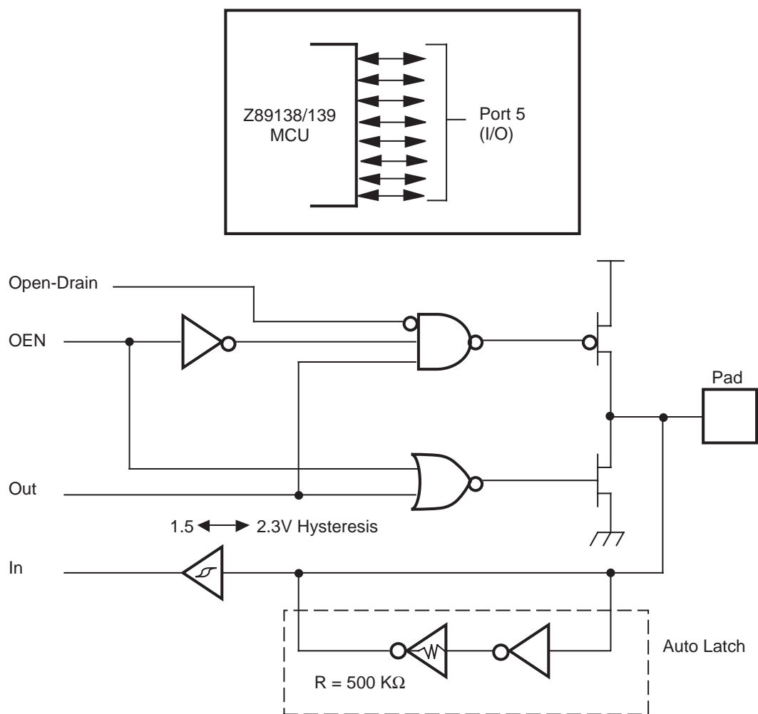
Figure 16. Port 5 Configuration
