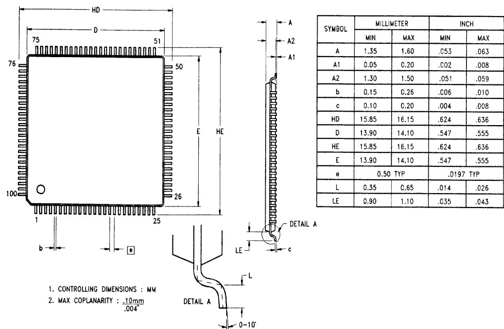
Figure 84. 100-Pin VQFP Package Diagram
