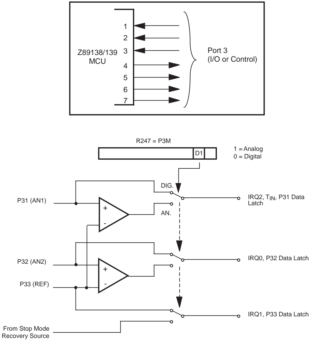
Figure 14. Port 3 Configuration
