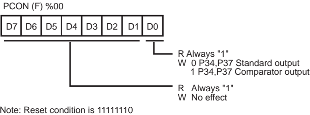
Figure 59. Port Configuration Register (PCON) (F) 00H [Write-Only]
