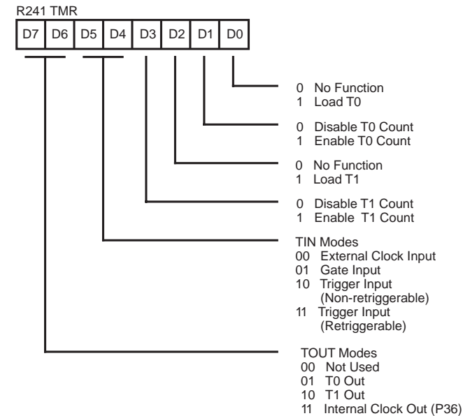
Figure 68. Timer Mode Register (F1H: Read/Write)
