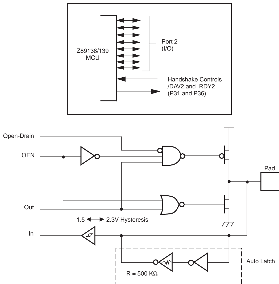
Figure 13. Port 2 Configuration
