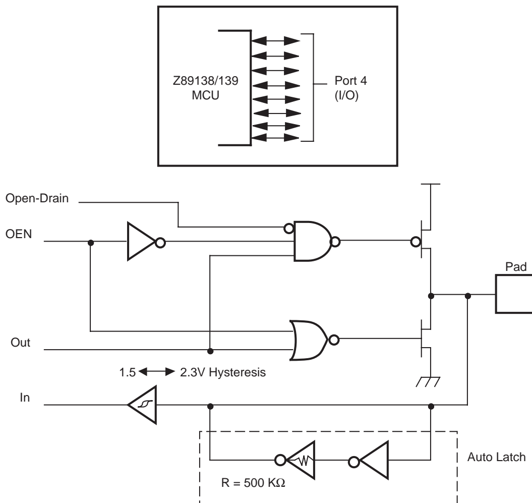
Figure 15. Port 4 Configuration
