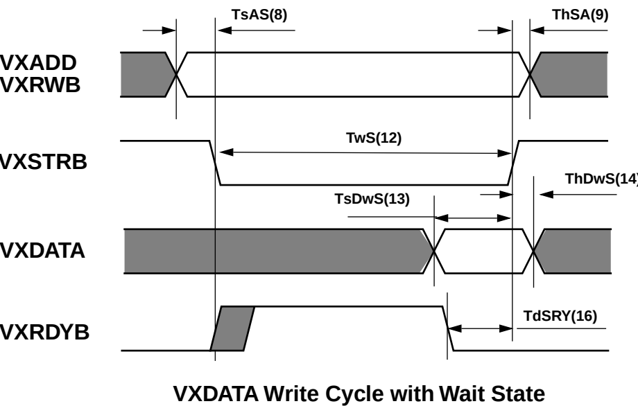
Figure 8. Read/Write Cycle Timing with Wait State
