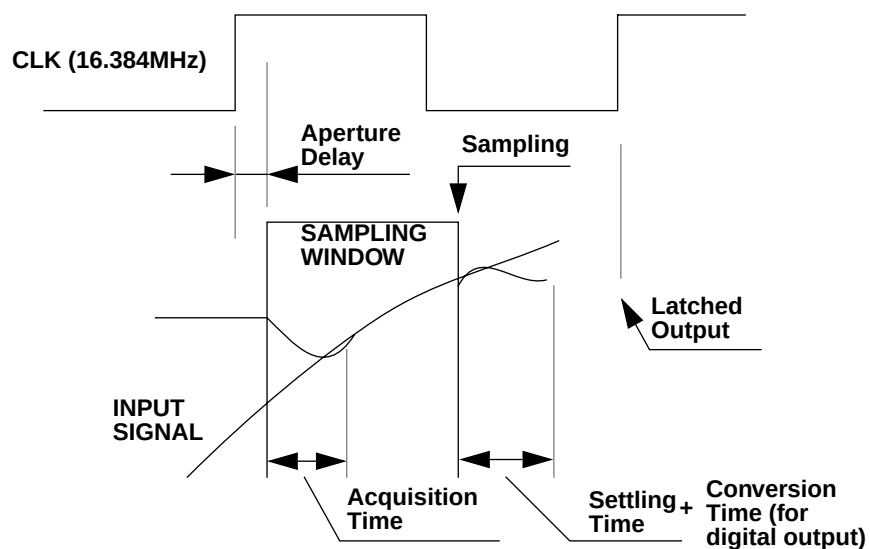
Figure 5. 1-Bit ADC Definition of Terms
