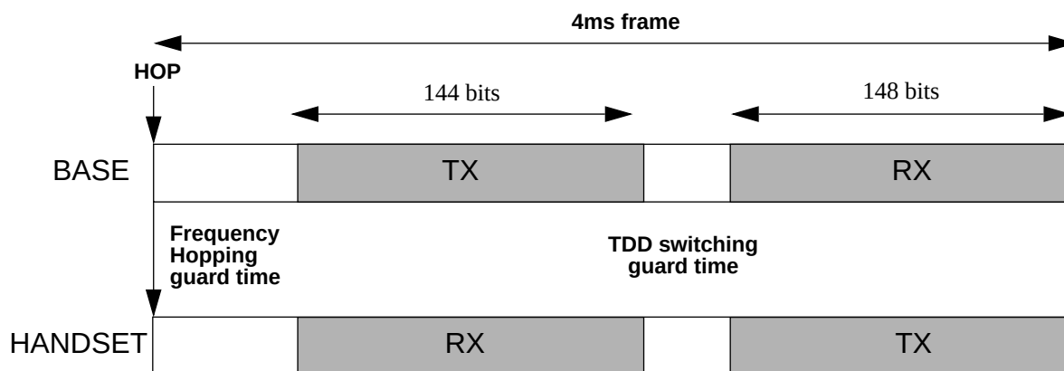
Figure 9. Basic Time Duplex Timing
