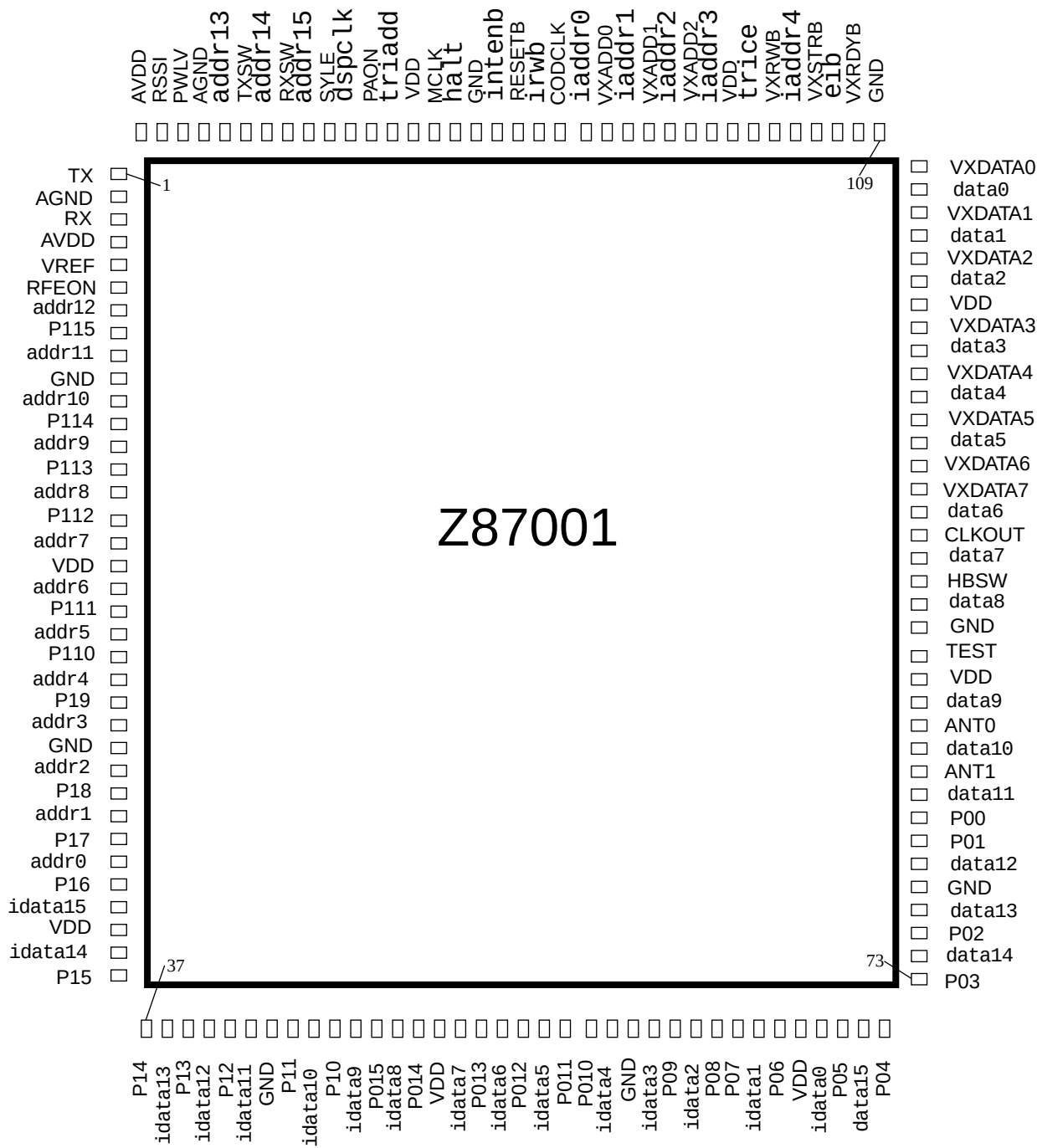
Figure 3. 144 Pin VQFP Pin Configuration
