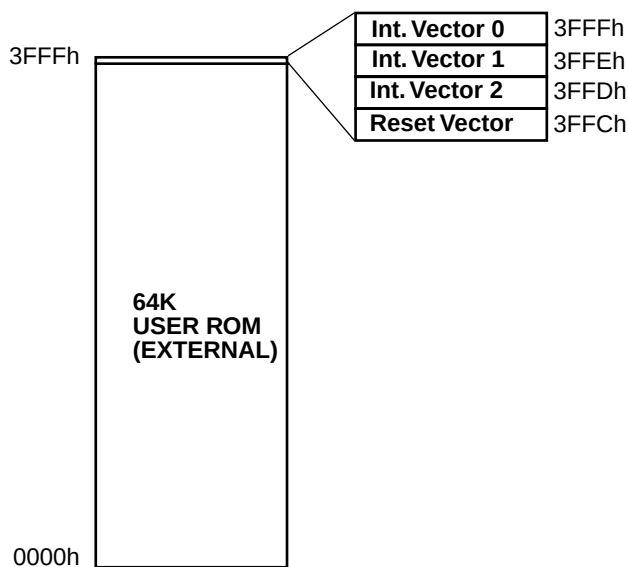
Figure 12. ROM Mapping
