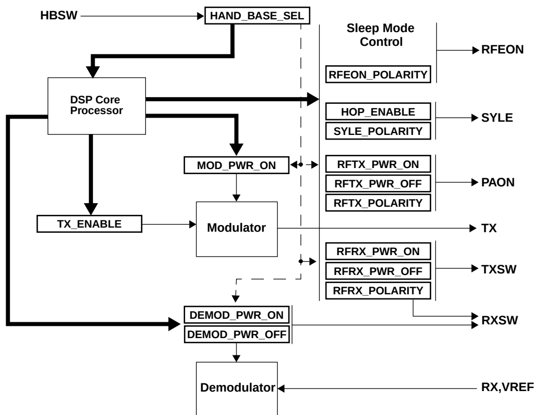
Figure 16. RF interface Control
