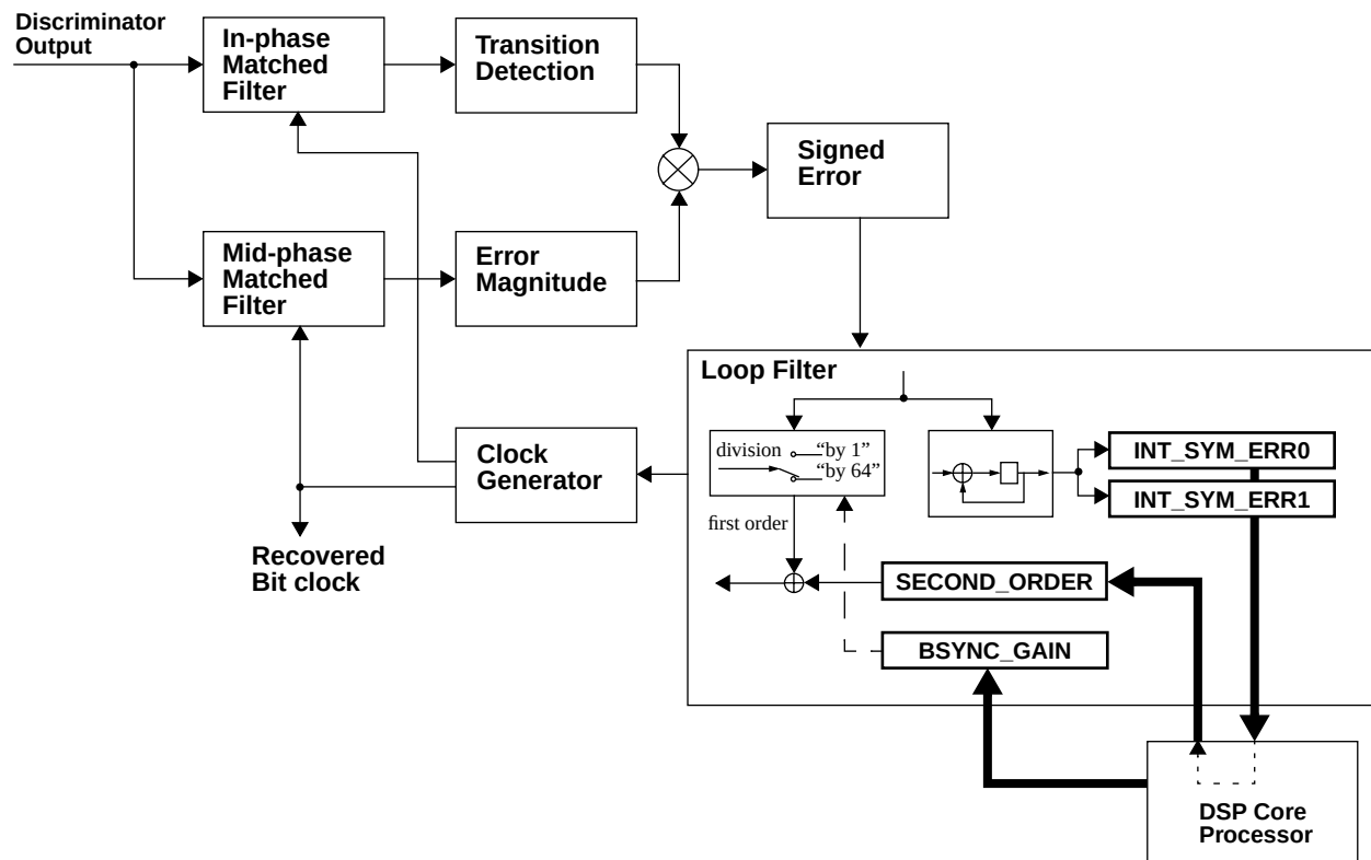
Figure 14. Bit Synchronizer Loop and Processor Control
