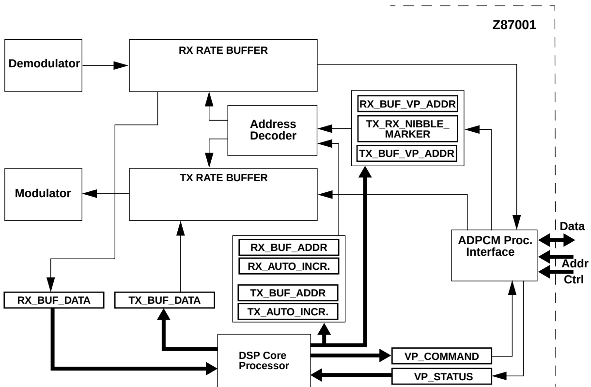
Figure 17. Rate Buffers Access and ADPCM Processor Interface
