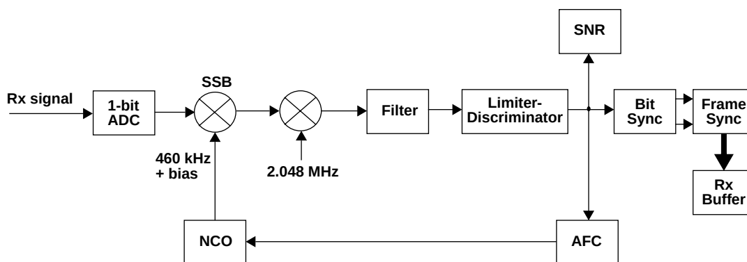
Figure 10. Demodulator Block Diagram
