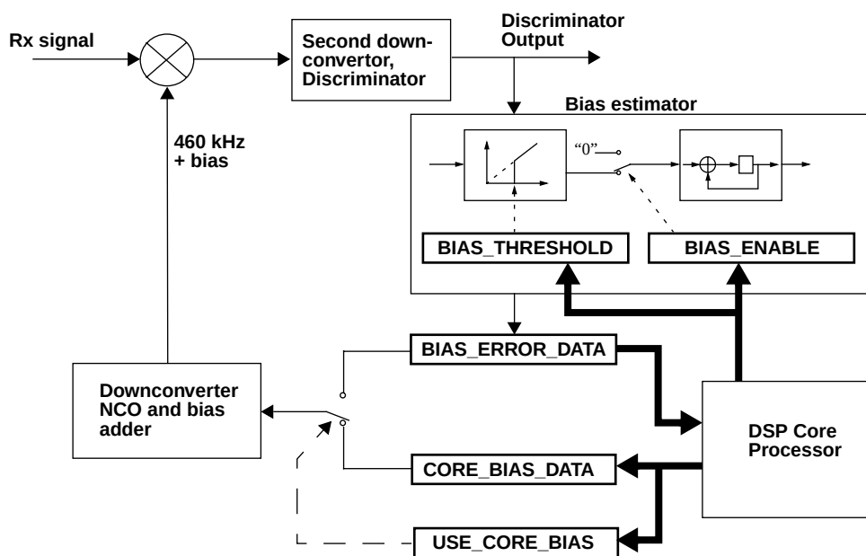
Figure 13. AFC Loop and Processor Control
