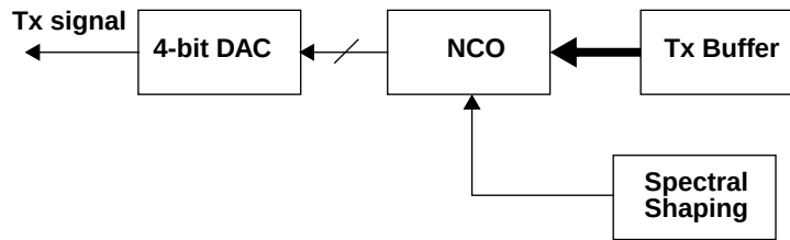
Figure 11. Modulator Block Diagram
