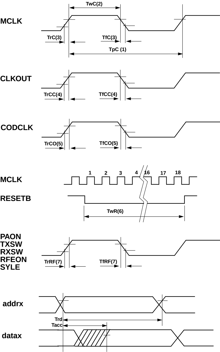
Figure 6. Transceiver Output Signal
