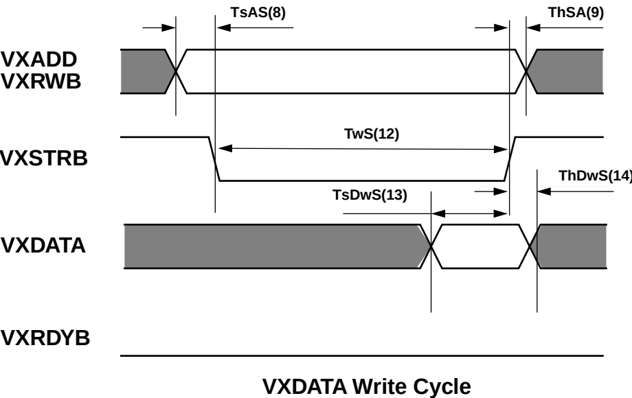
Figure 7. Read/Write Cycle Timings
