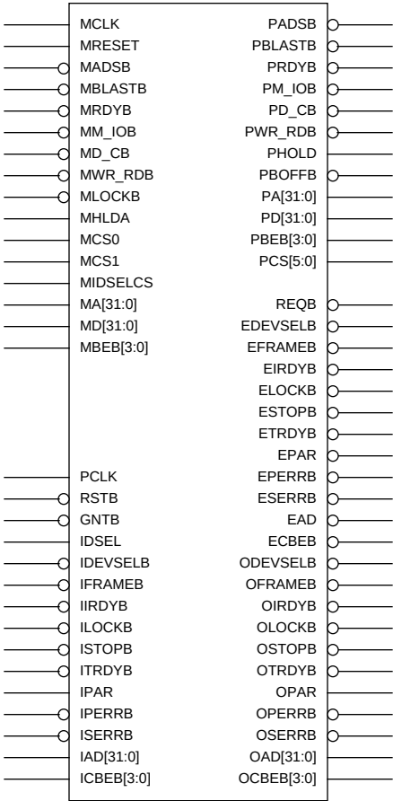
Figure 203. Logic Symbol
