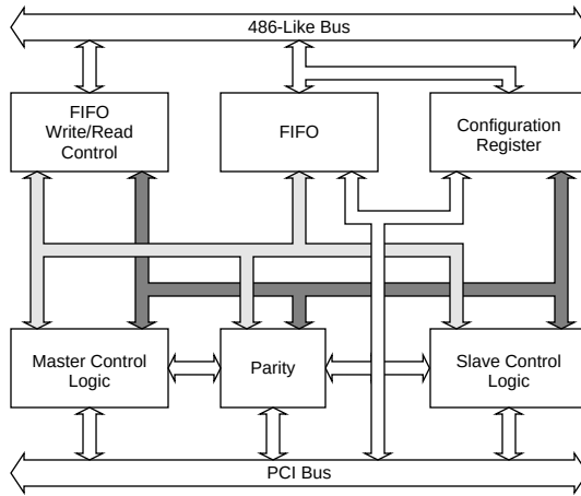
Figure 204. PCI Mega Macrocell Block Diagram
