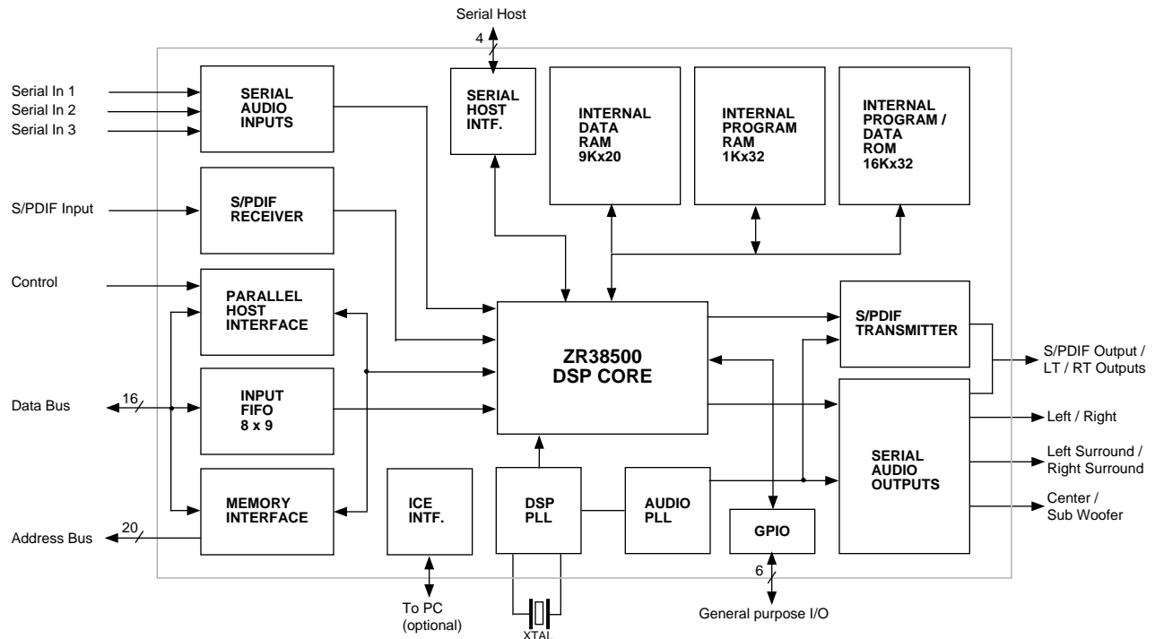
Figure 1. ZR38600 - Functional Block Diagram
