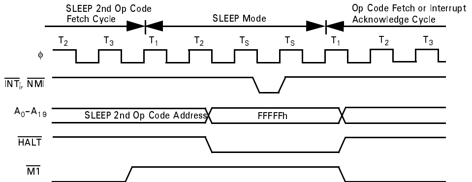
Figure 14. SLEEP Timing
