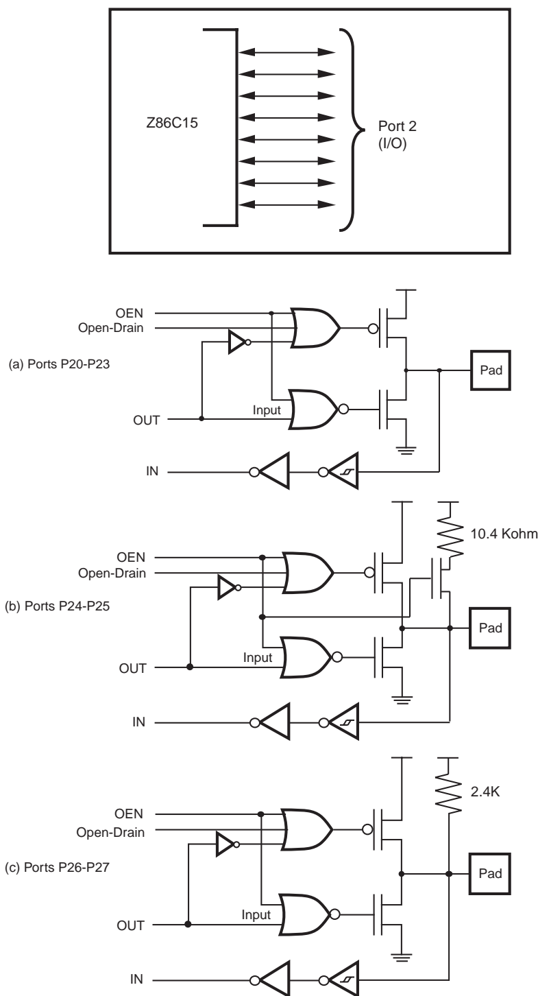
Figure 9. Port 2 Configuration
