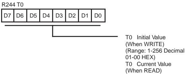
Figure 25. Counter/Timer 0 Register (F4H: Read/Write)
