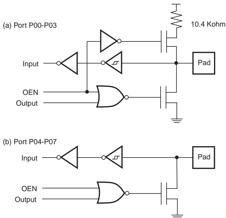
Figure 7. Port 0 Configuration
