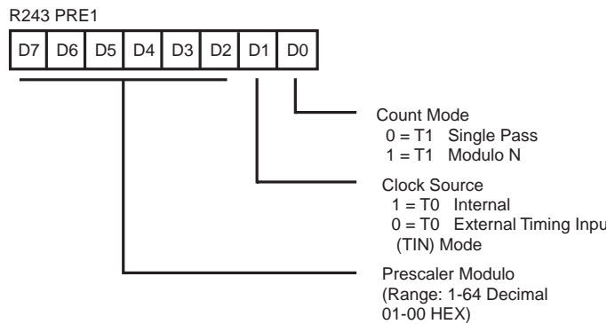
Figure 24. Prescaler 1 Register (F3H: Write Only)
