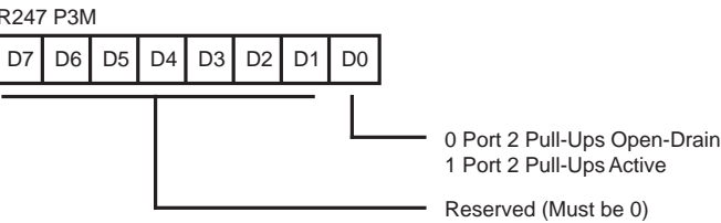
Figure 28. Port 3 Mode Register (F7H: Write Only)
