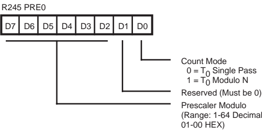
Figure 26. Prescaler 0 Register (F5H: Write Only)
