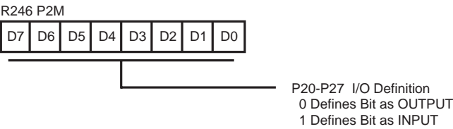
Figure 27. Port 2 Mode Register (F6H: Write Only)
