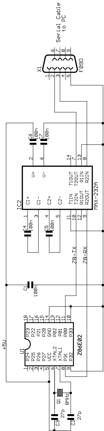
Figure 4. RS-232 Setup
