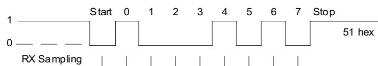
Figure 1. Basic 8-bit UART Protocol
