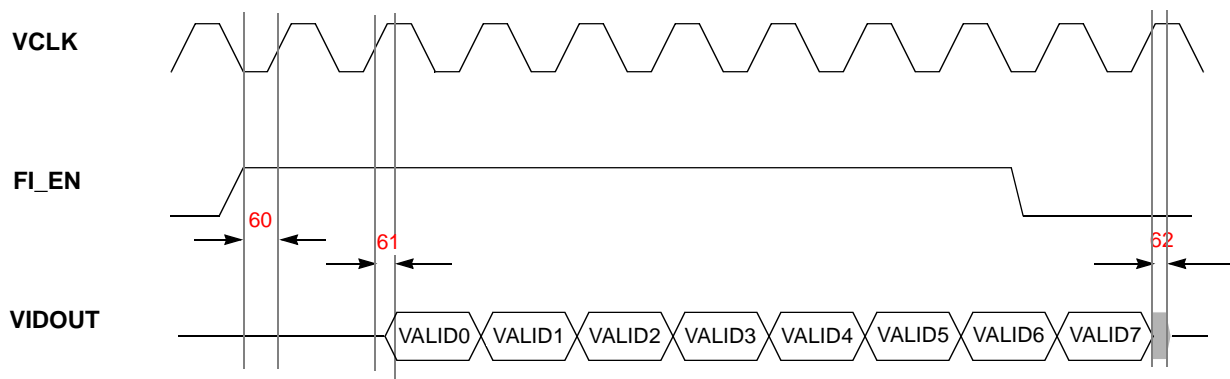
Figure 48. Video output in Enabled Mode
