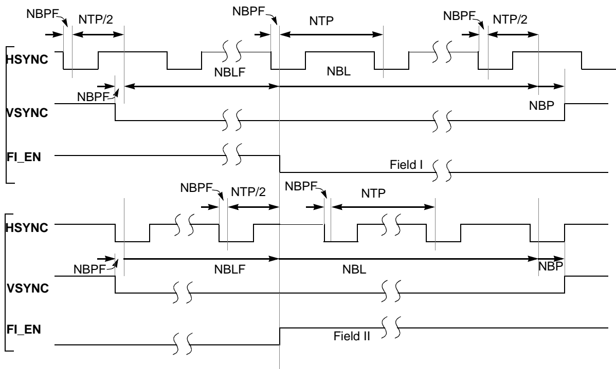
Figure 21. Field Index: (long HSYNC, long VSYNC, width of NBL is non-integer number of lines)
