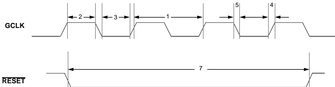
Figure 35. GCLK and \overline{\text{RESET}} timing
