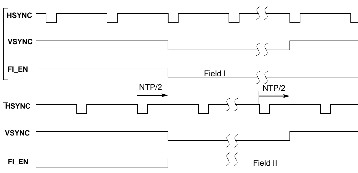
Figure 14. Field Index: (short HSYNC, short VSYNC, width of VSYNC is integer number of lines)
