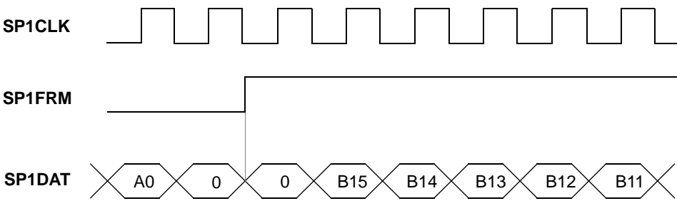
Figure 23. Beginning of serial port frame with transition frame sync signal, length of previous frame is 18 clocks
