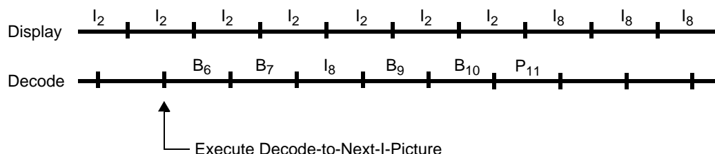
Figure 32. Decode-to-Next-I-Picture
