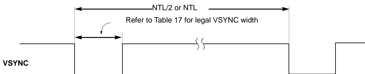
Figure 10. Input VSYNC
