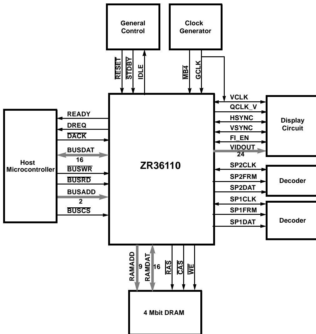
Figure 3. Generic ZR36110 Schematic Diagram
