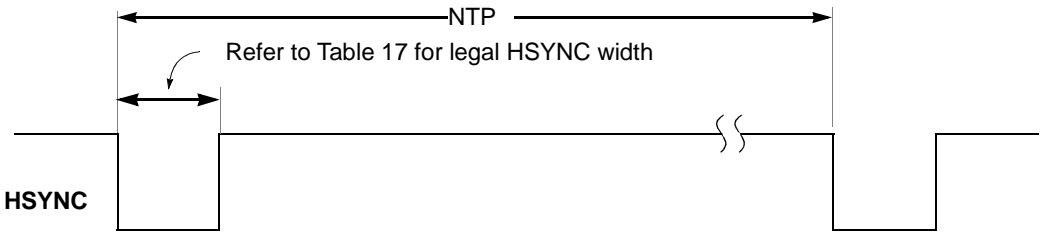
Figure 7. Input HSYNC
