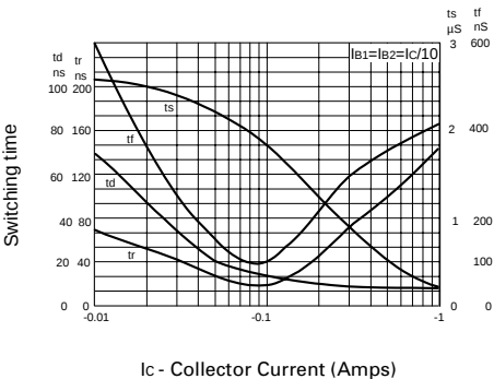
Switching Speeds
