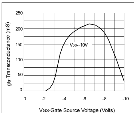
Transconductance v gate-source voltage
