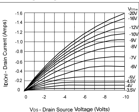
Saturation Characteristics
