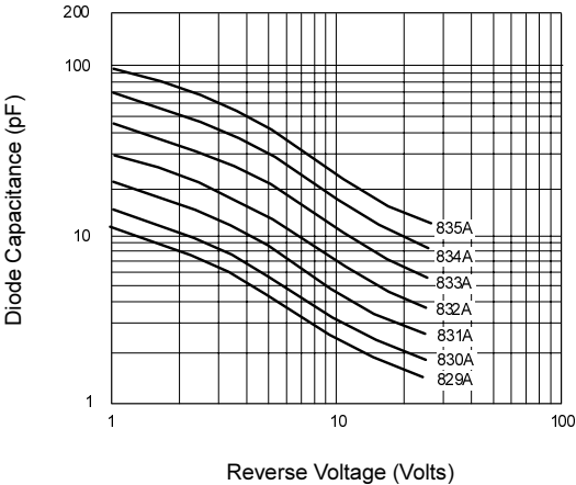
Diode Capacitance
