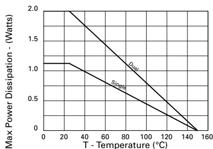
Derating curve
