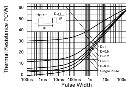
Transient Thermal Resistance Q1 and Q3 or Q2 and Q4 "On"
