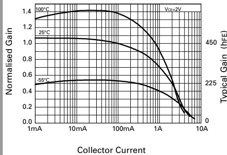
h_{FE} vs I_C
