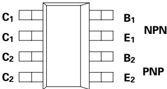
PARTMARKING DETAIL – T6702
