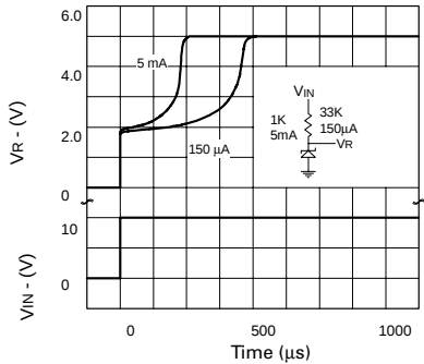
Transient Response (Single Pulse)
