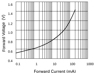
Forward Characteristics
