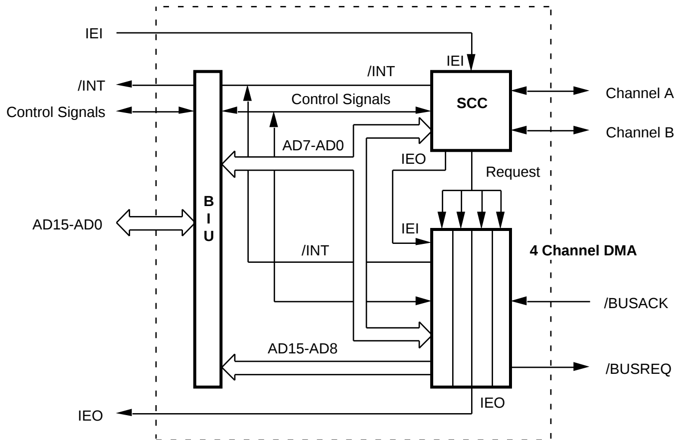
Z16C35 Functional Block Diagram
