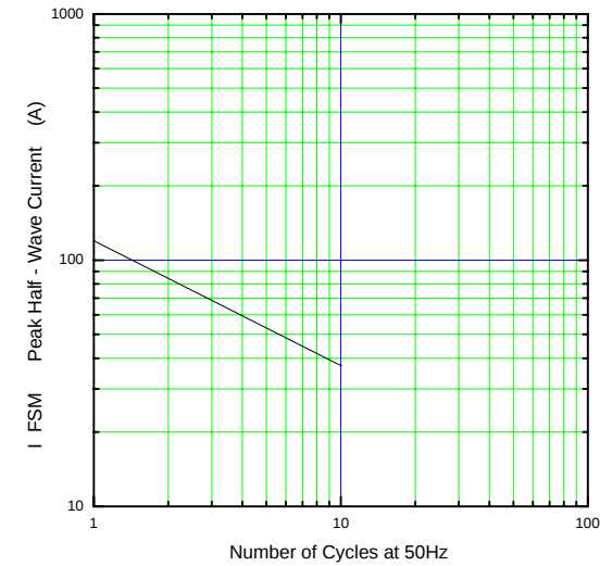
Surge Capability
