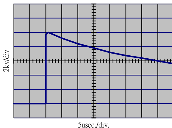
10kv Fig-1.Lightning Original Waveform
