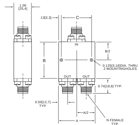
FIGURE 2 SERIES YL-N
