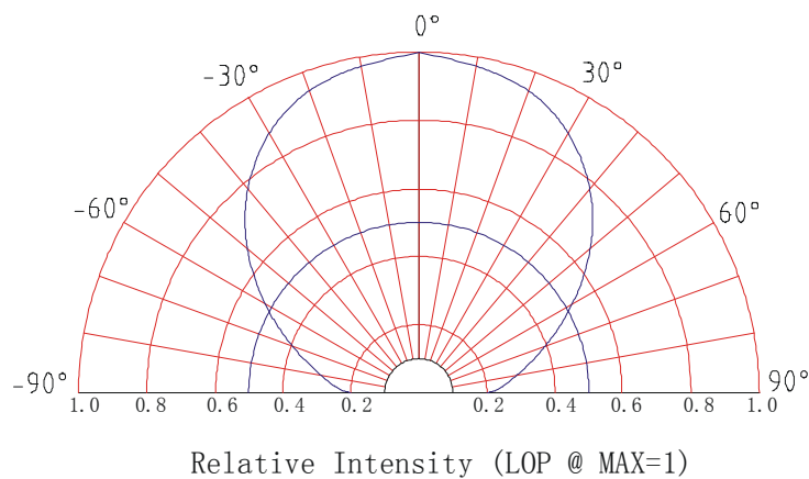
Beam Pattern
