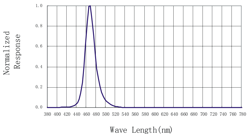
Spectral Radiance ( Peak @ 468nm)
