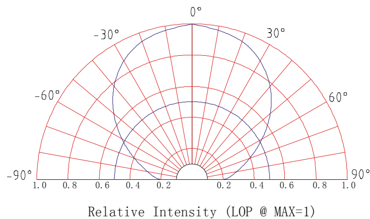
Beam Pattern
