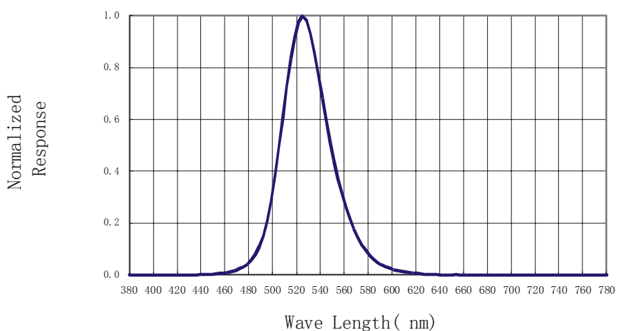
Spectral Radiance (Peak @ 525nm)
