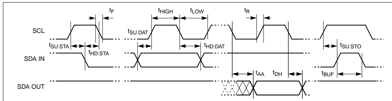
Figure 4. Bus Timing
