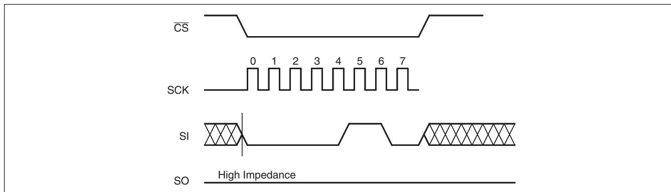
Figure 8. Write Sequence
