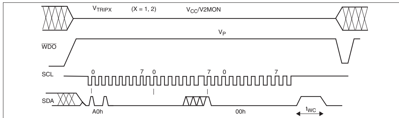
Figure 4. Watchdog Restart
