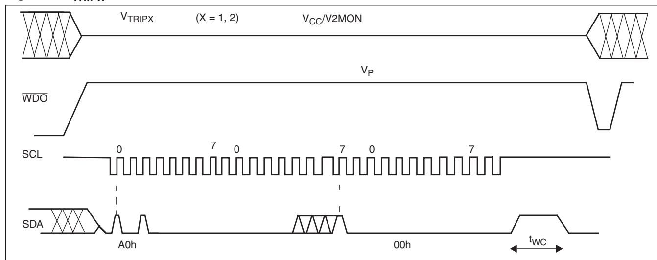
Figure 2. V_{TBIPX} Set/Reset Conditions
