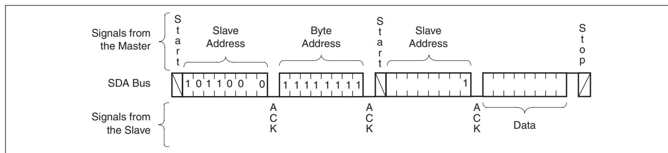
Figure 9. Read Sequence
