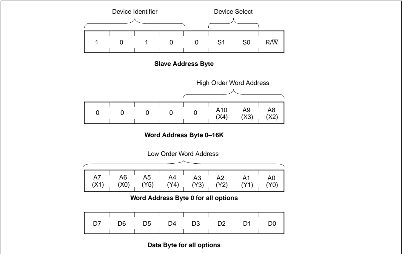
Figure 15. X4163/5 Addressing
