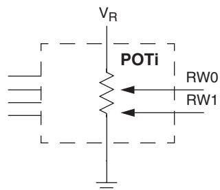
Four terminal Potentiometer; Variable voltage divider
