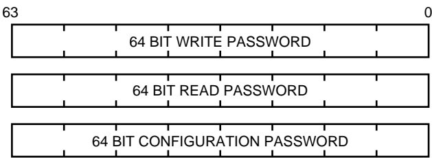
Figure 2. Password Registers
