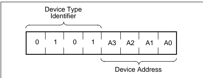
Figure 1. Slave Address
