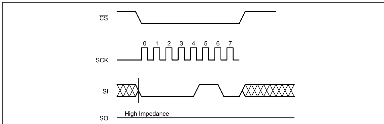
Figure 10. Write Sequence
