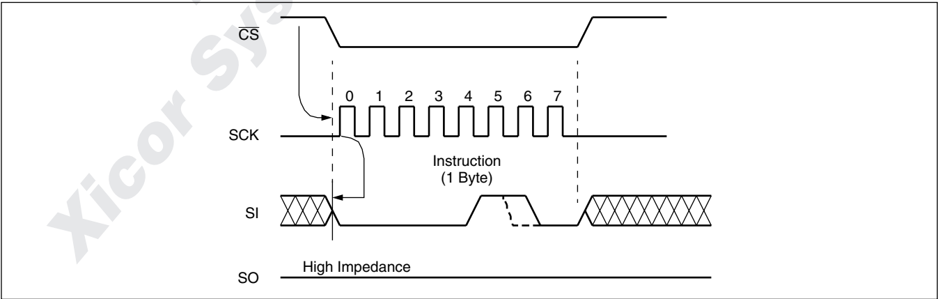
Figure 3. WREN/WRDI Sequence
