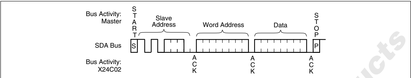
Figure 5. Byte Write
