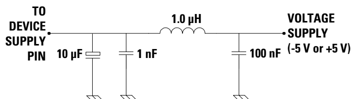
Figure 3. Filter Network
