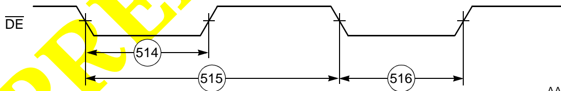
Figure 2-43 OnCE—Debug Request
