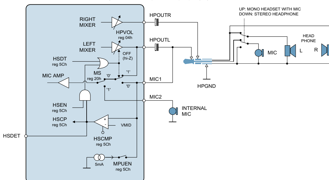
Figure 10 Headset Autodetect
